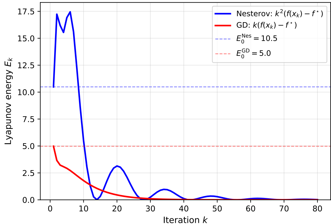
Lyapunov Energies (bounded \Rightarrow rate confirmed)
