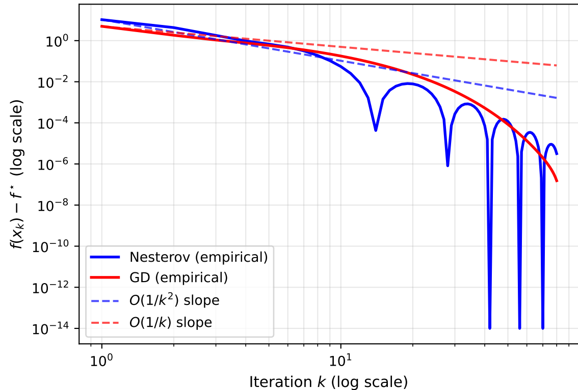
Nesterov vs. GD: Convergence Rates (Benchmark~B, log-log scale)
