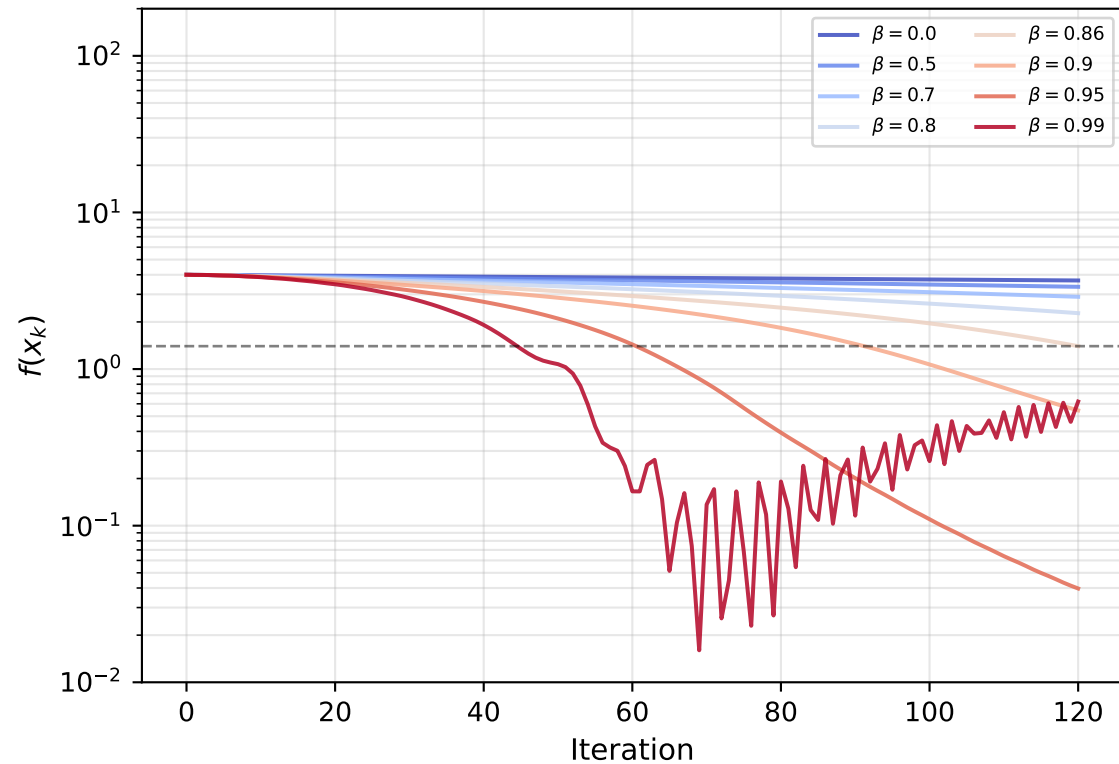
Heavy Ball on Rosenbrock: Varying \beta ( \alpha = 0.0008 , 120 iters)
