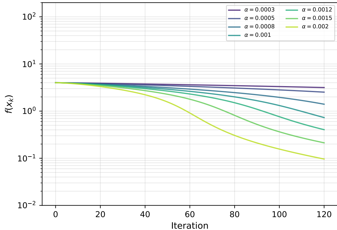
Heavy Ball on Rosenbrock: Varying \alpha ( \beta = 0.86 , 120 iters)
