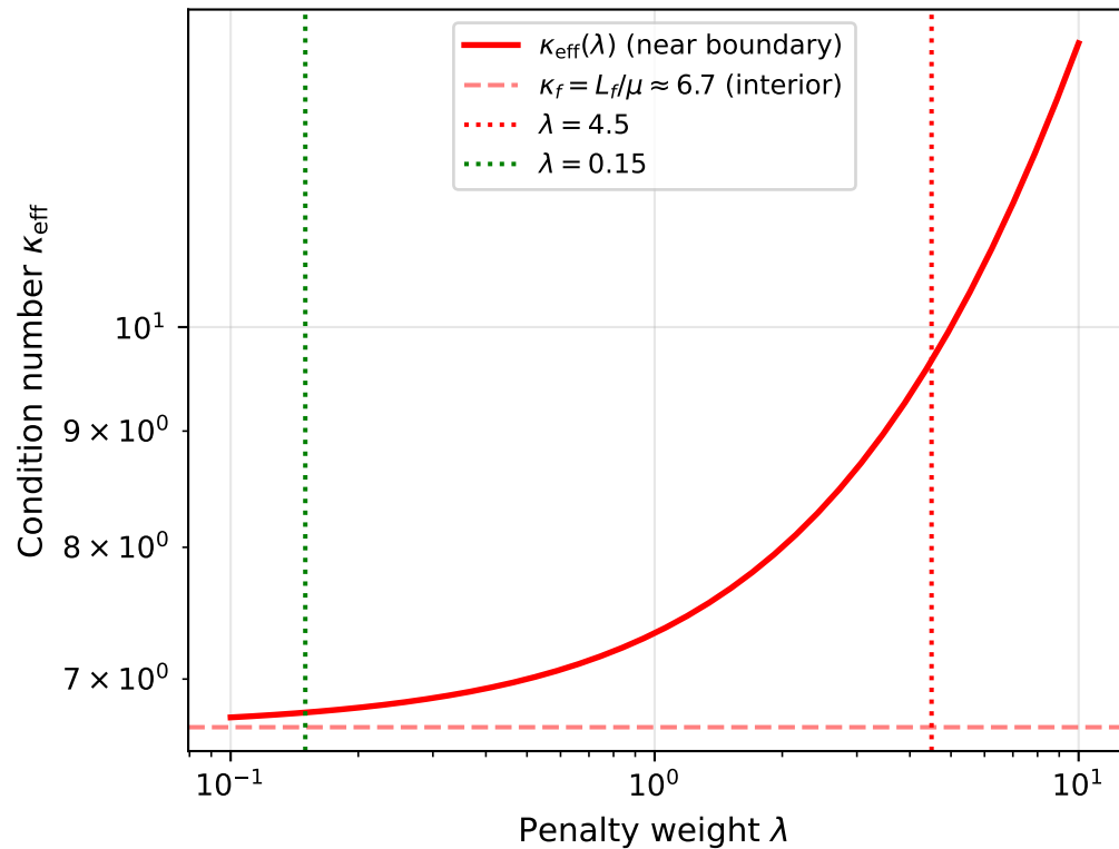
Condition number growth with penalty weight
