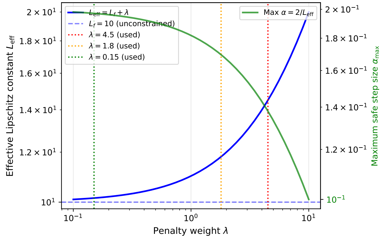
Growth of effective Lipschitz constant
