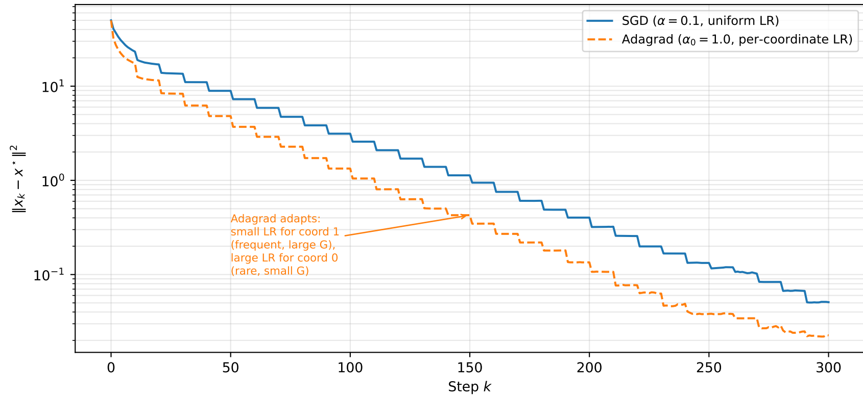
Adagrad vs SGD on a Sparse Gradient Problem (coord 0 updates 10× rarer)
