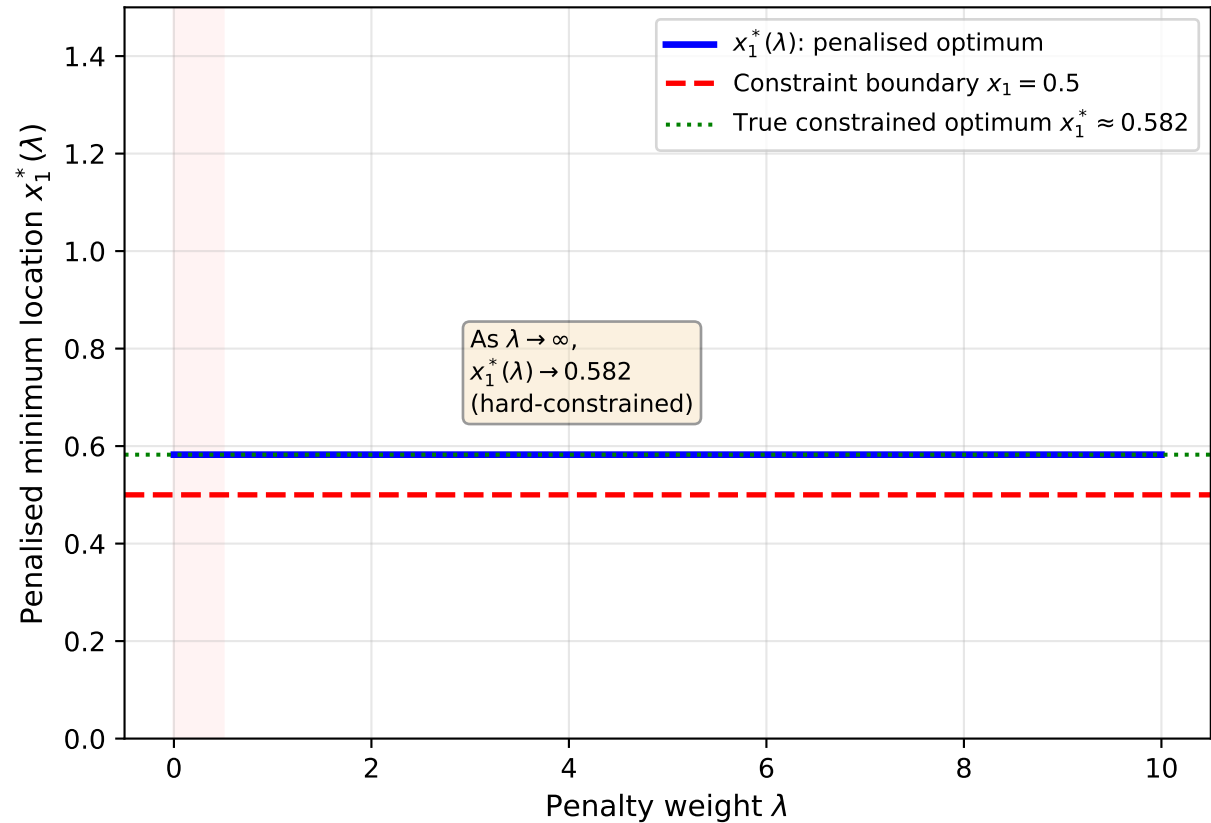
Q5: How Penalty Drives Solution Toward Constraint Boundary
