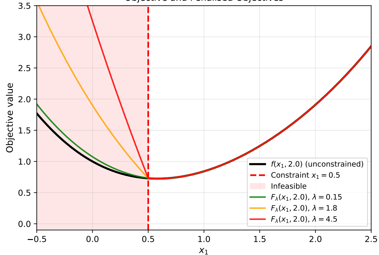
Q5: Cross-section ( x_2 = 2 ) of Objective and Penalised Objectives
