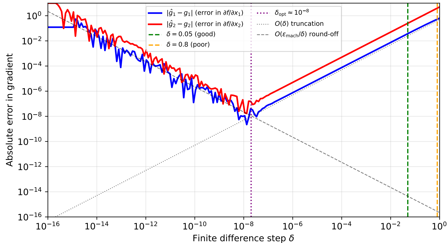
Finite Difference Gradient Approximation Error vs \delta (Benchmark B at x = (0.5, 3.0) )
