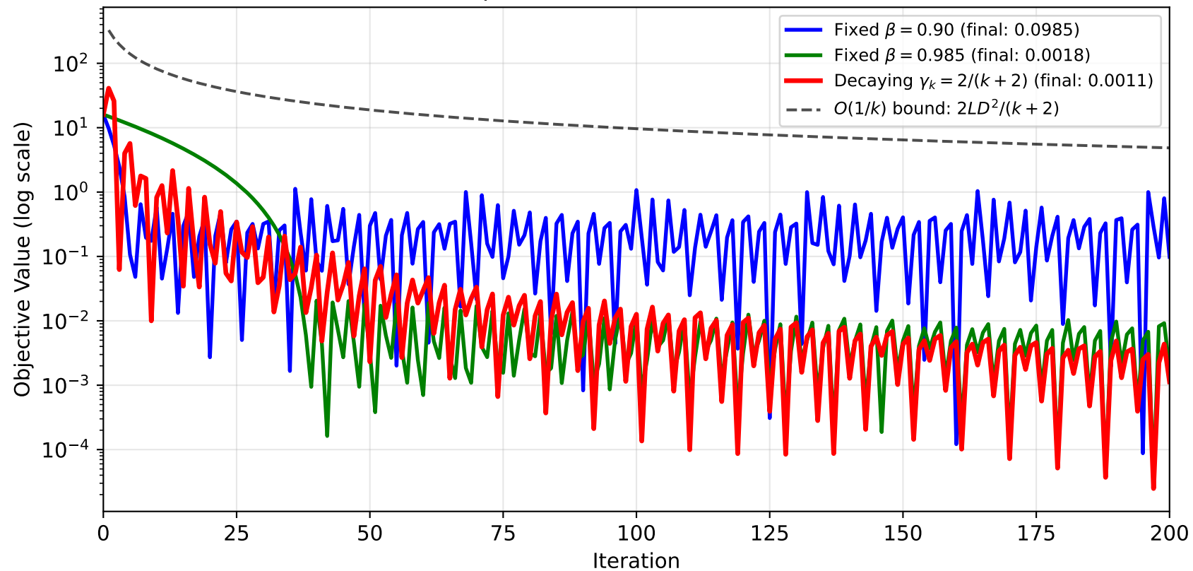
Q6: Frank--Wolfe Convergence — Fixed \beta vs Decaying \gamma_k = 2/(k + 2) (Interior Optimum: f(x) = (x_1 - 1)^2 + (x_2 - 5)^2 )
