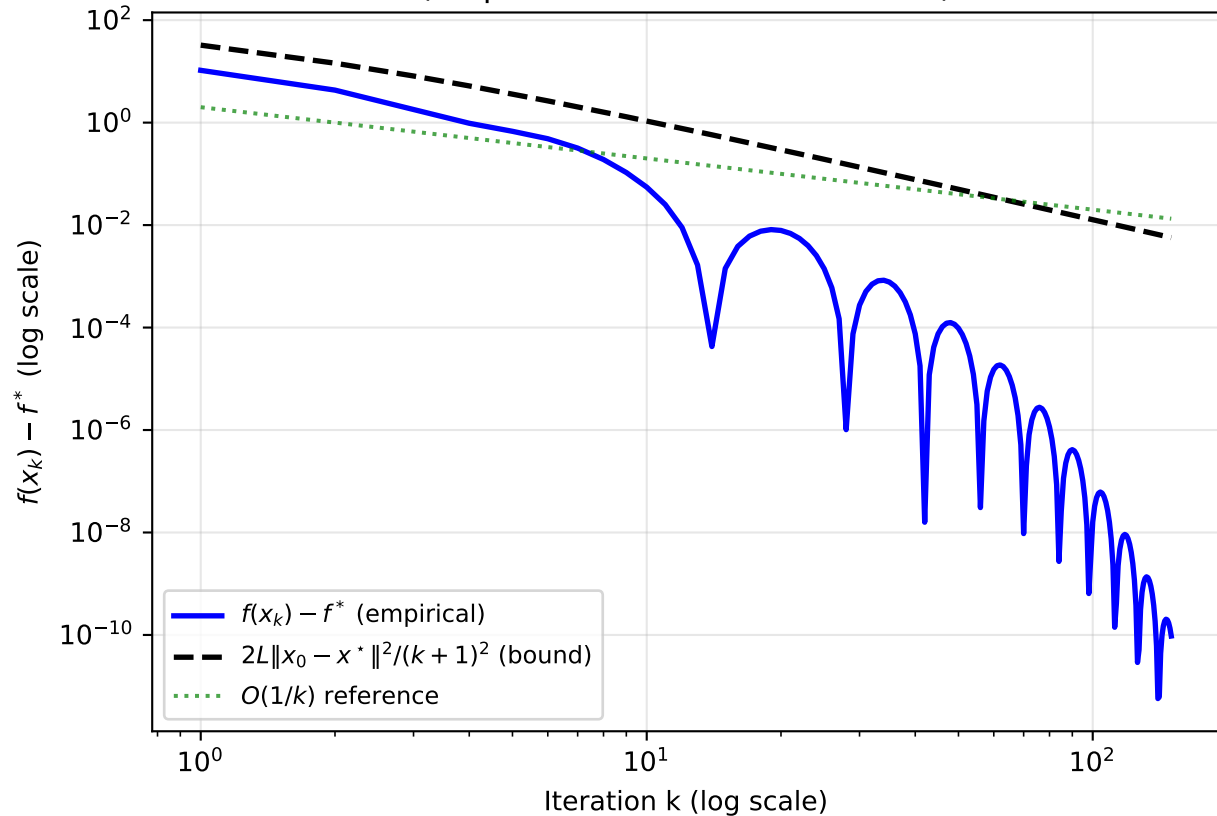
Nesterov Convergence vs Theoretical Bound (empirical faster than the bound)
