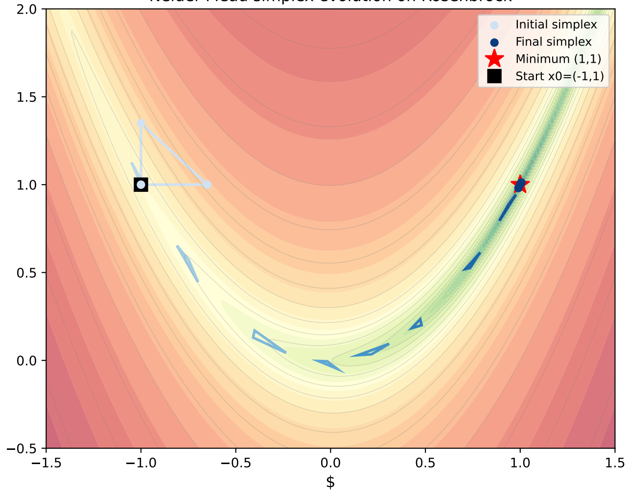
Nelder-Mead simplex evolution on Rosenbrock
