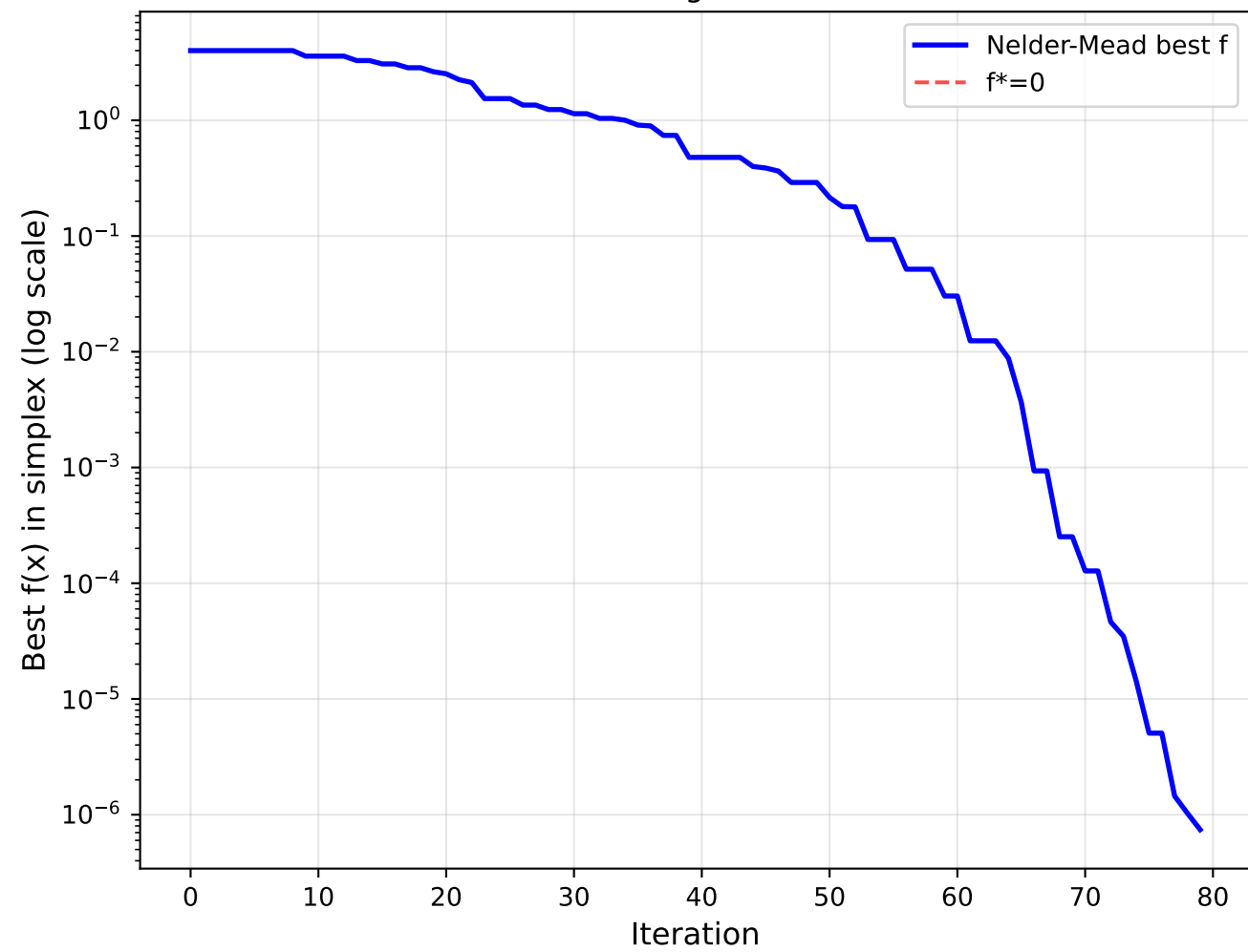
Nelder-Mead convergence on Rosenbrock
