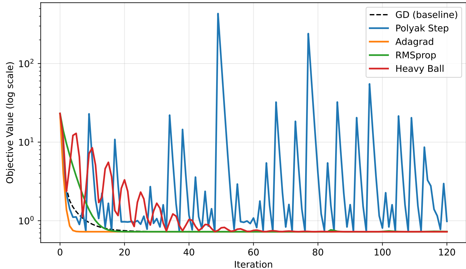
Q1: Convergence Comparison — Benchmark B (Toy Neural Network)
