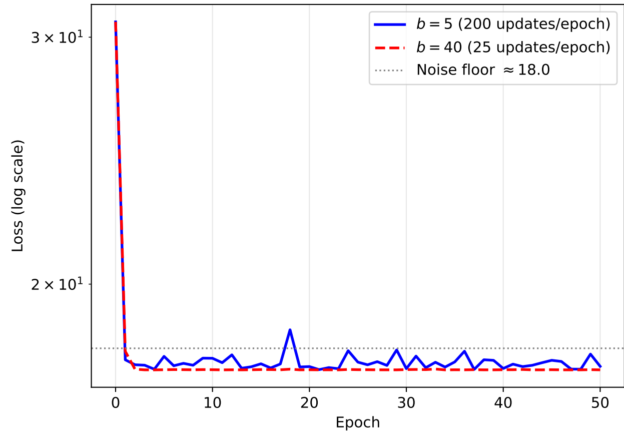
Q2: Mini-Batch SGD, \sigma = 6 (6 \times noise)
