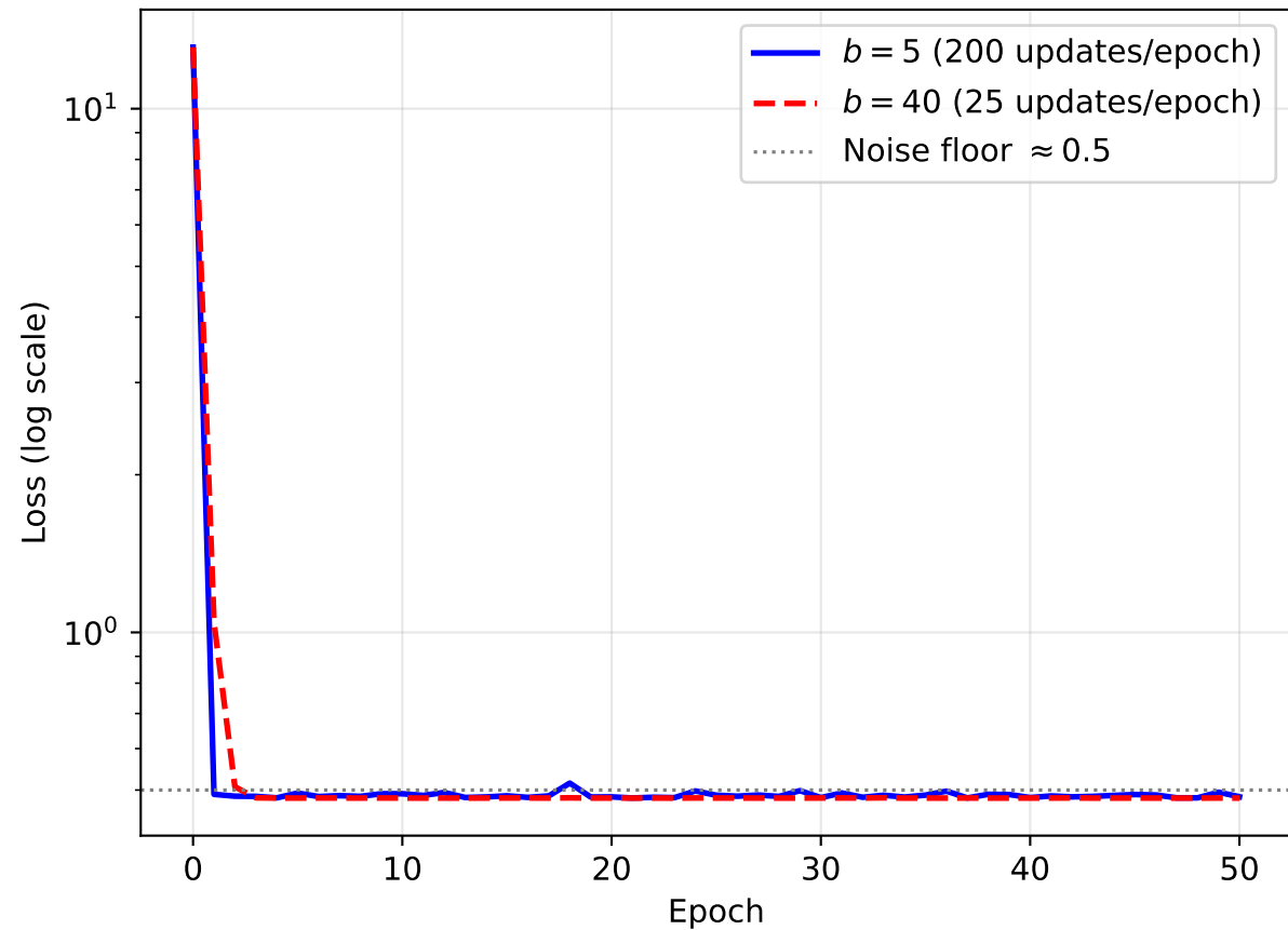
Q2: Mini-Batch SGD, \sigma = 1 (original noise)
