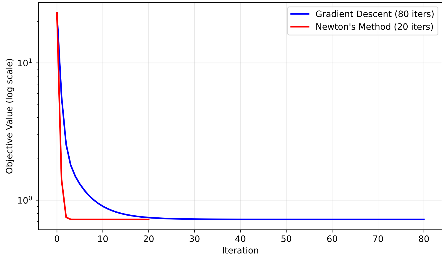
Q3: Newton vs GD — Benchmark B (Toy Neural Network)
