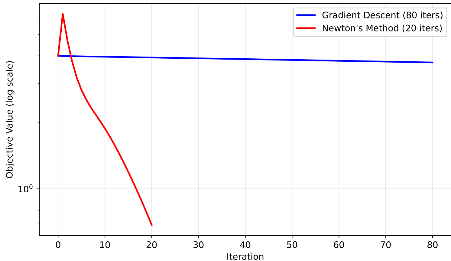
Q3: Newton vs GD — Benchmark C (Rosenbrock)
