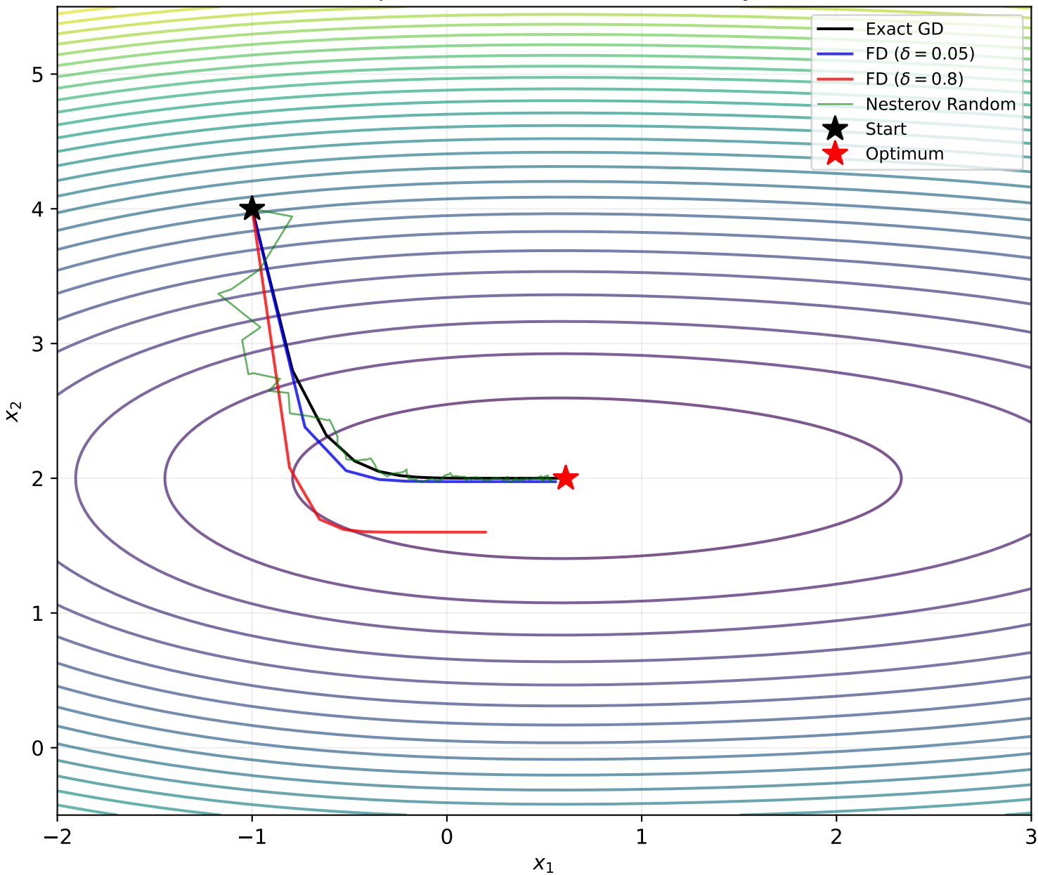
Q4A: Trajectories on Benchmark B (Toy NN)
