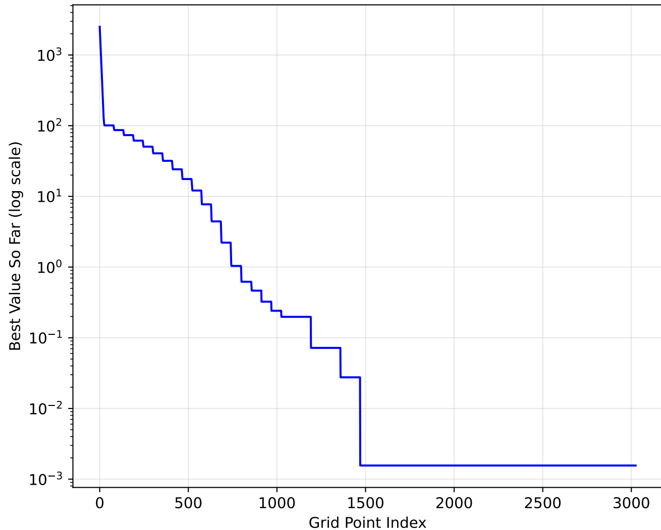
Q4B: Grid Search Best-So-Far (best f = 0.0016 )
