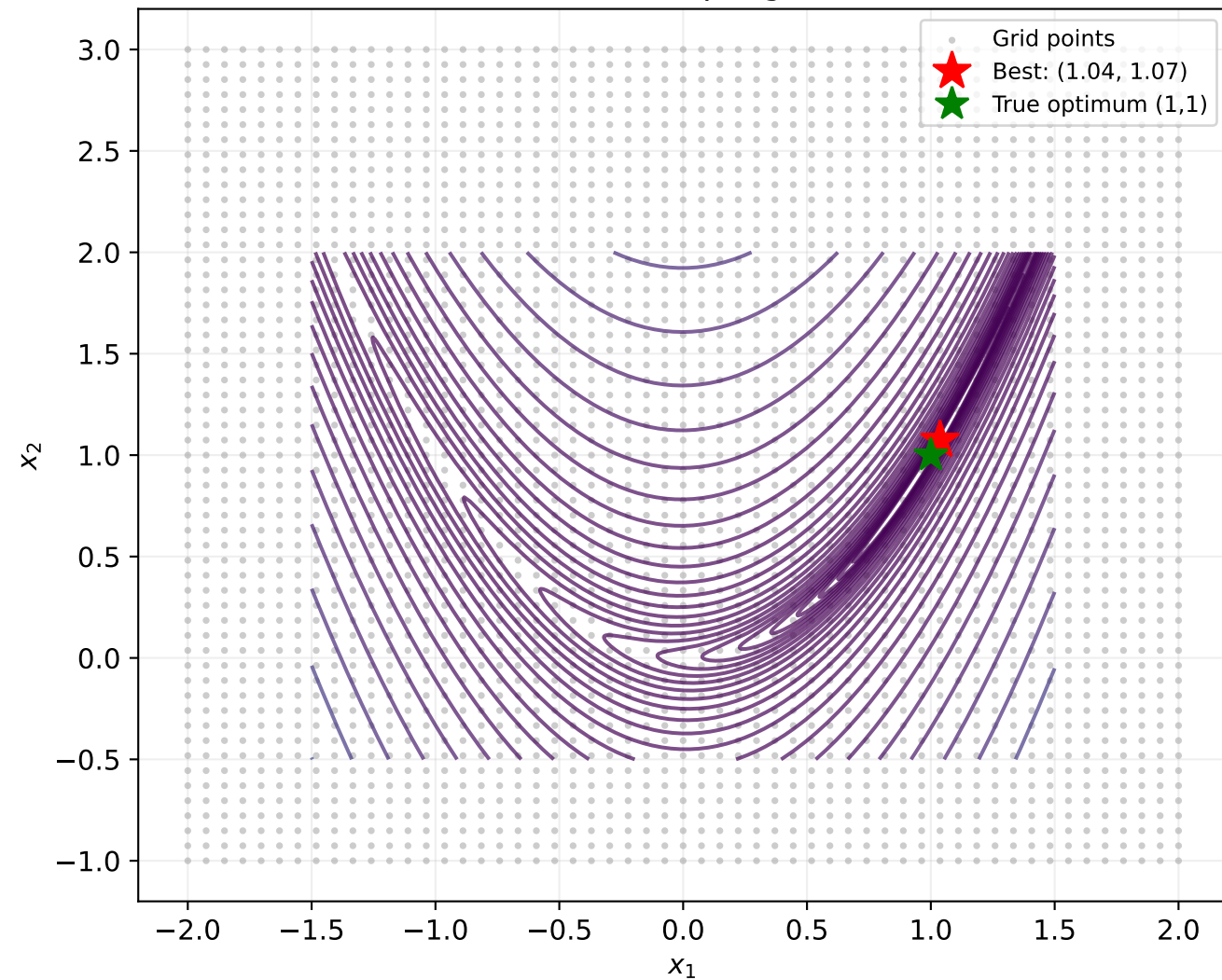
Q4B: Grid Search Sampling — Rosenbrock
