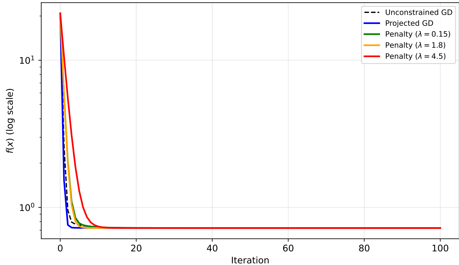
Q5: Objective Value vs Iteration
