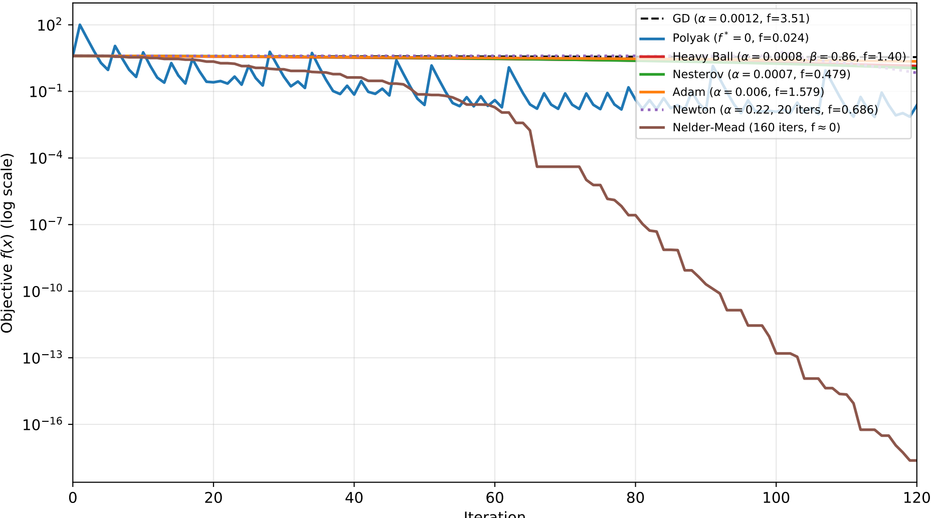
Summary: All Key Methods on Benchmark C (Rosenbrock, \kappa \approx 2508 )
