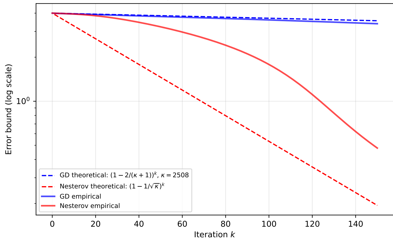
Theoretical vs Empirical Rates (Benchmark C, \kappa \approx 2508 )
