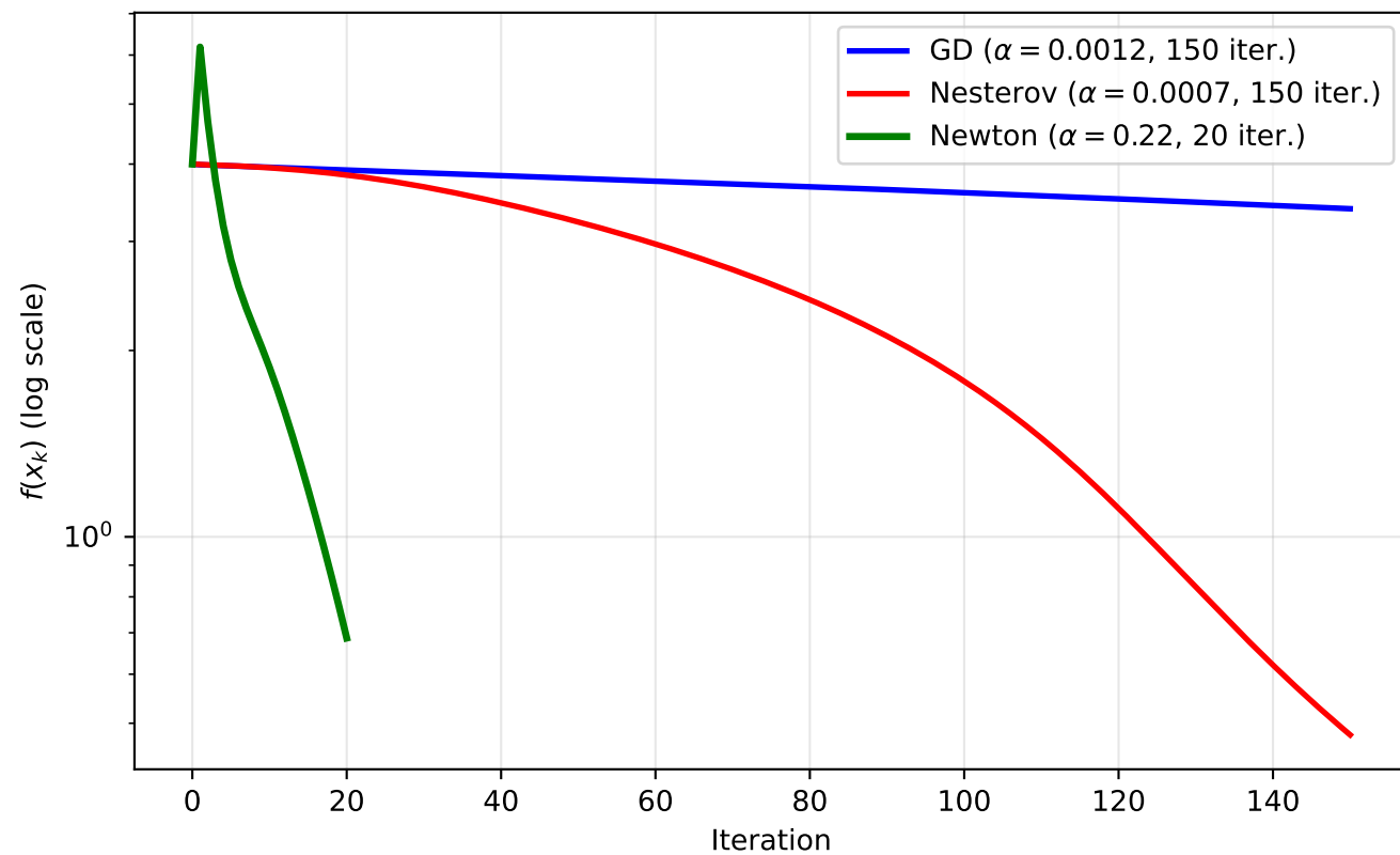
Benchmark C: GD vs Nesterov vs Newton
