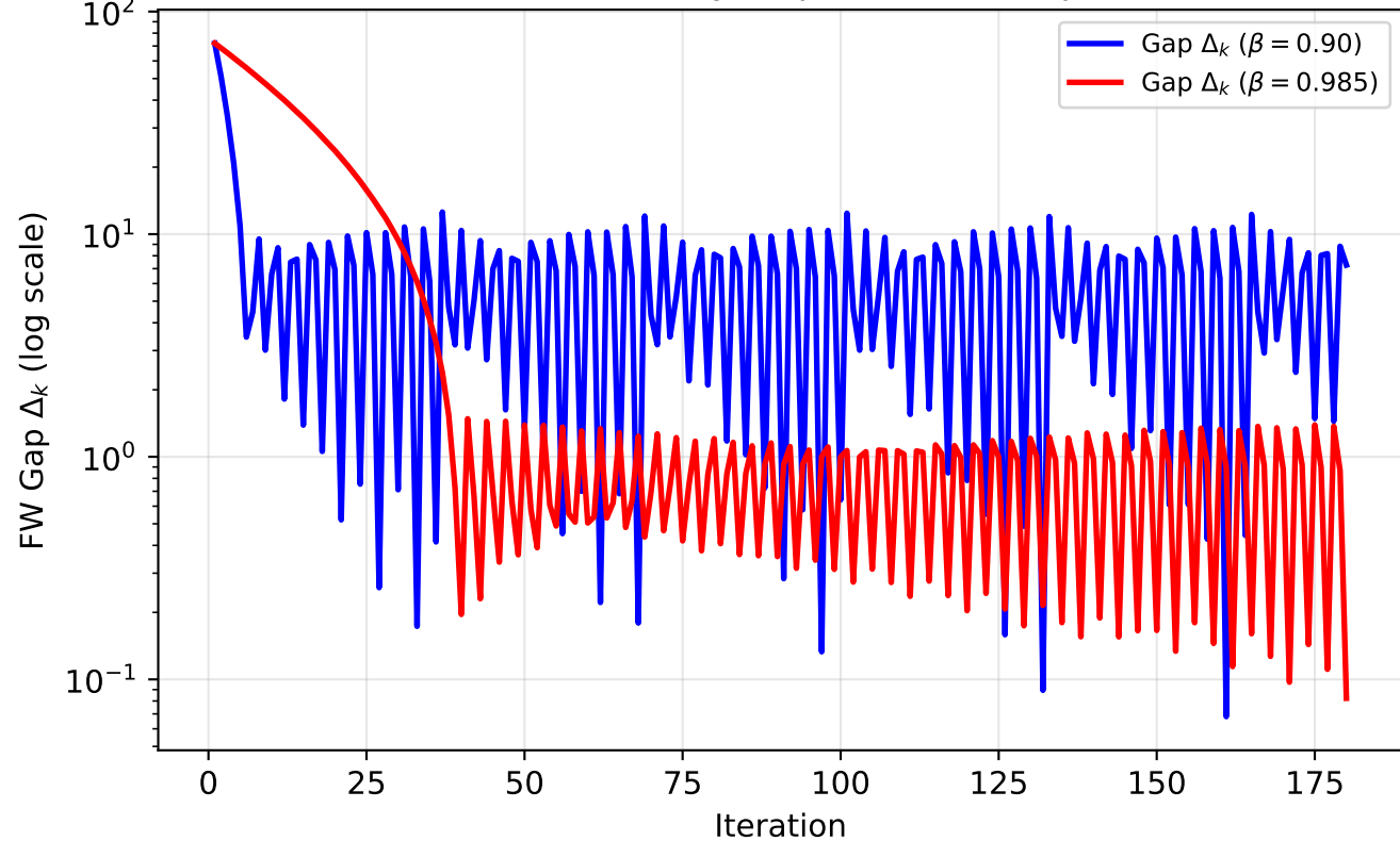
Frank--Wolfe Duality Gap — Interior Optimum
