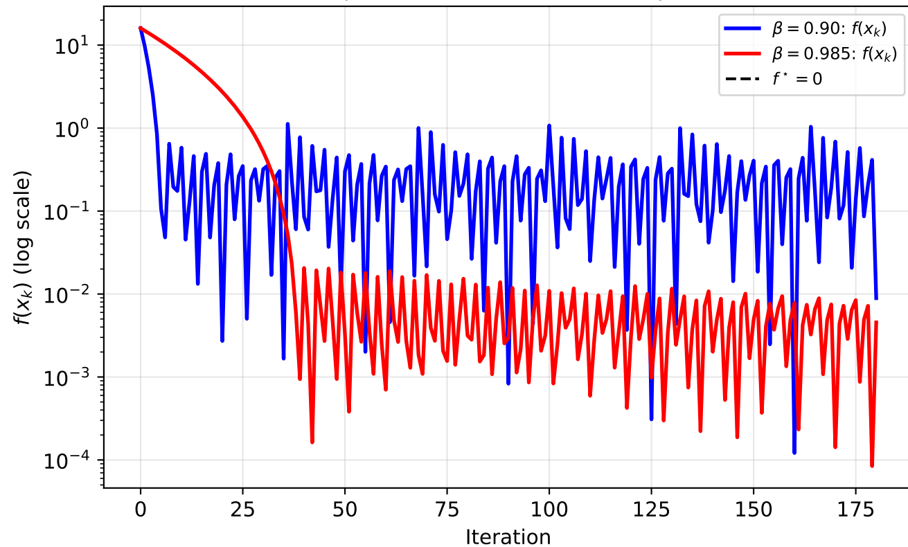
FW Objective Value — Interior Optimum
