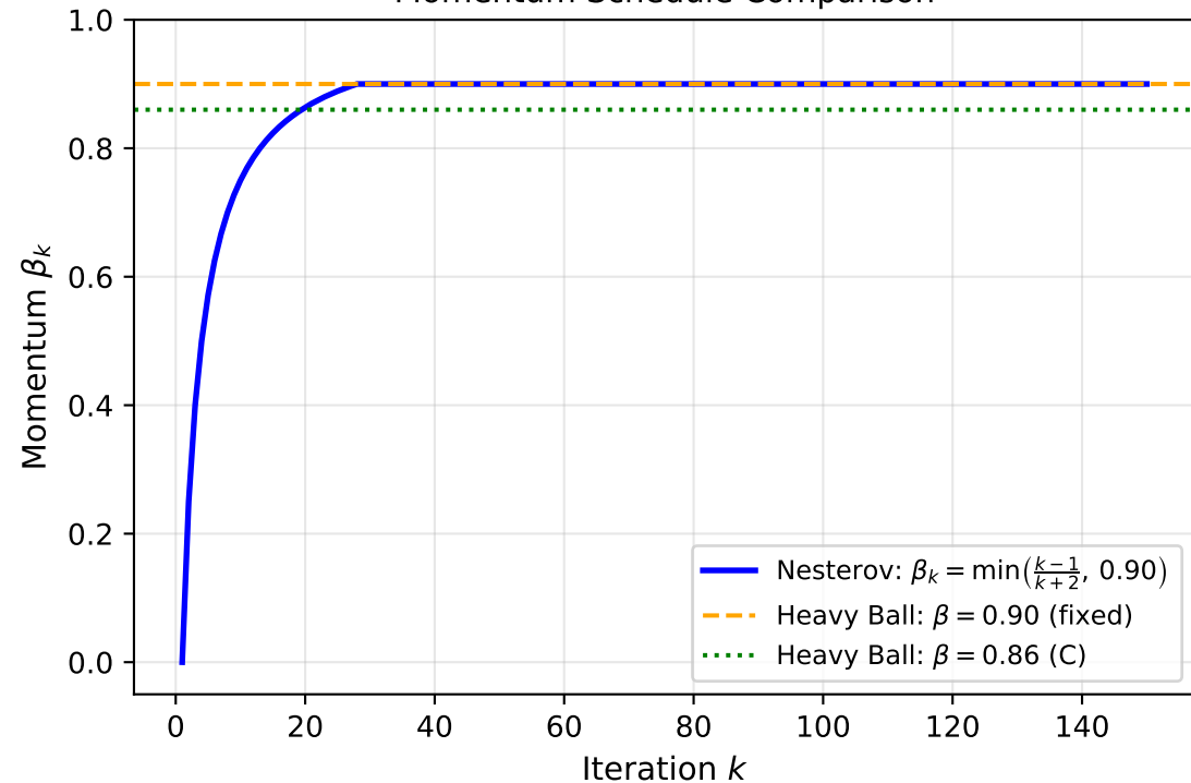
Momentum Schedule Comparison
