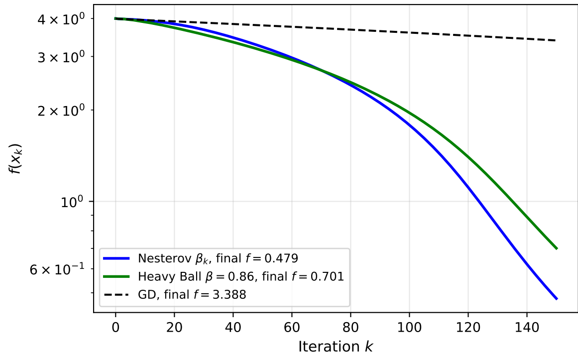
Convergence on Benchmark C (Rosenbrock)
