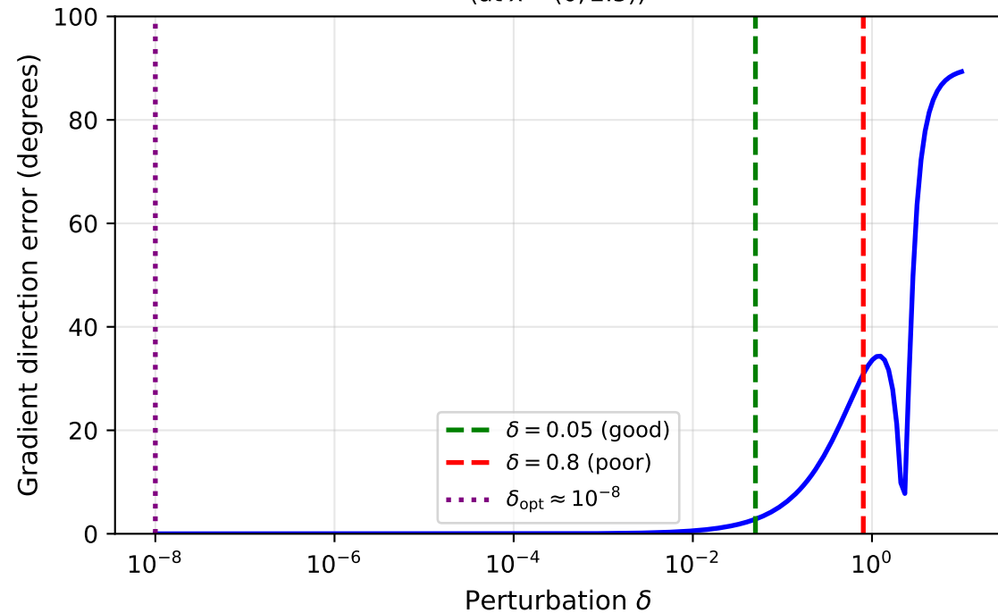
FD Gradient Direction Error on Rosenbrock (at x = (0, 2.5) )
