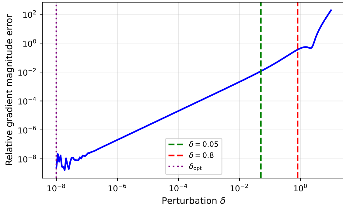
FD Gradient Magnitude Error on Rosenbrock
