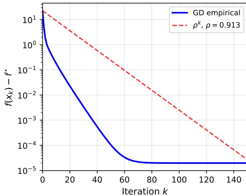
Benchmark B (Toy Neural Network) \kappa \approx 3.5\text{--}6.9, L = 10
