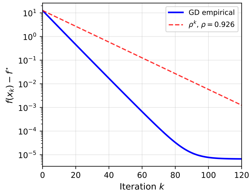
Benchmark A (Linear Regression) \kappa \approx 1.12, L \approx 1.03
