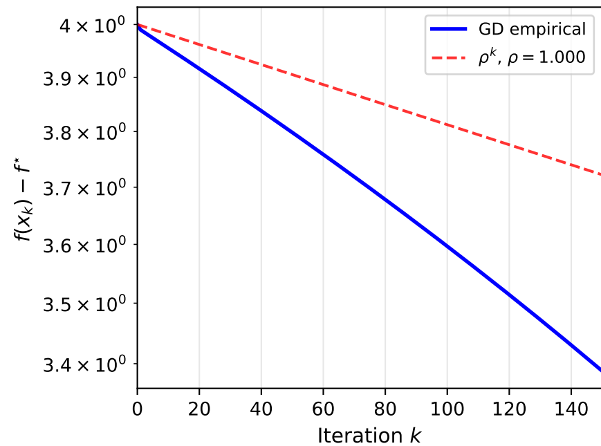
Benchmark C (Rosenbrock) \kappa \approx 2508, L \approx 1002
