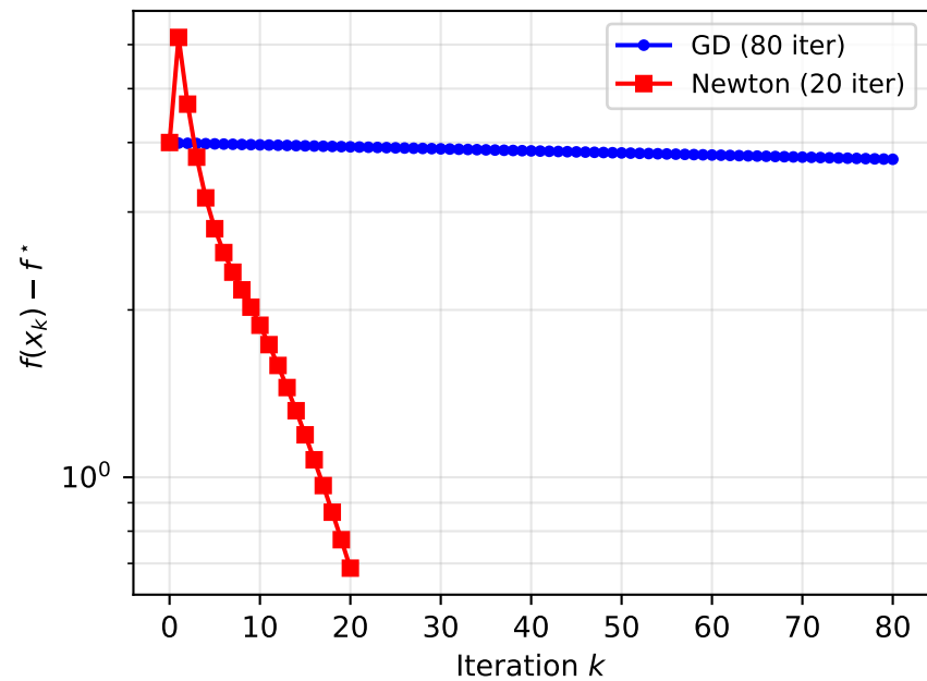
Benchmark C (Rosenbrock, \kappa \approx 2504 )
