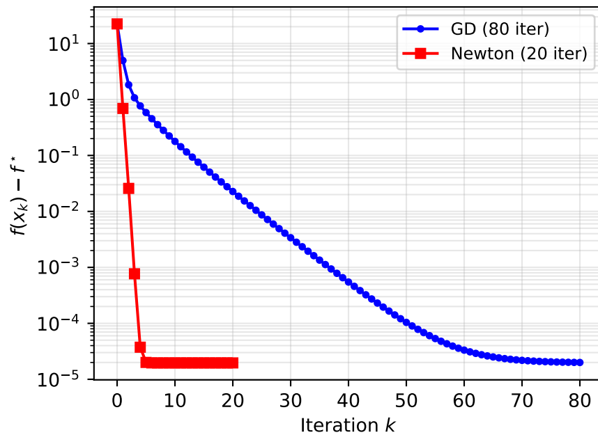
Benchmark B (NN loss, \kappa \approx 7 )
