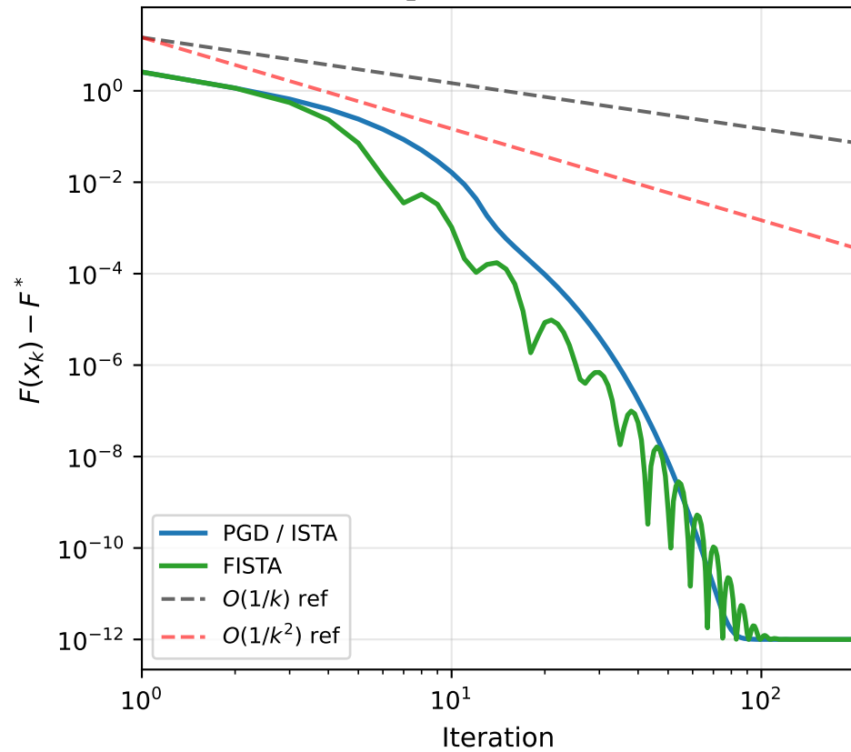
FISTA vs PGD on LASSO \min \frac{1}{2}\|Ax - b\|^2 + \lambda\|x\|_1
