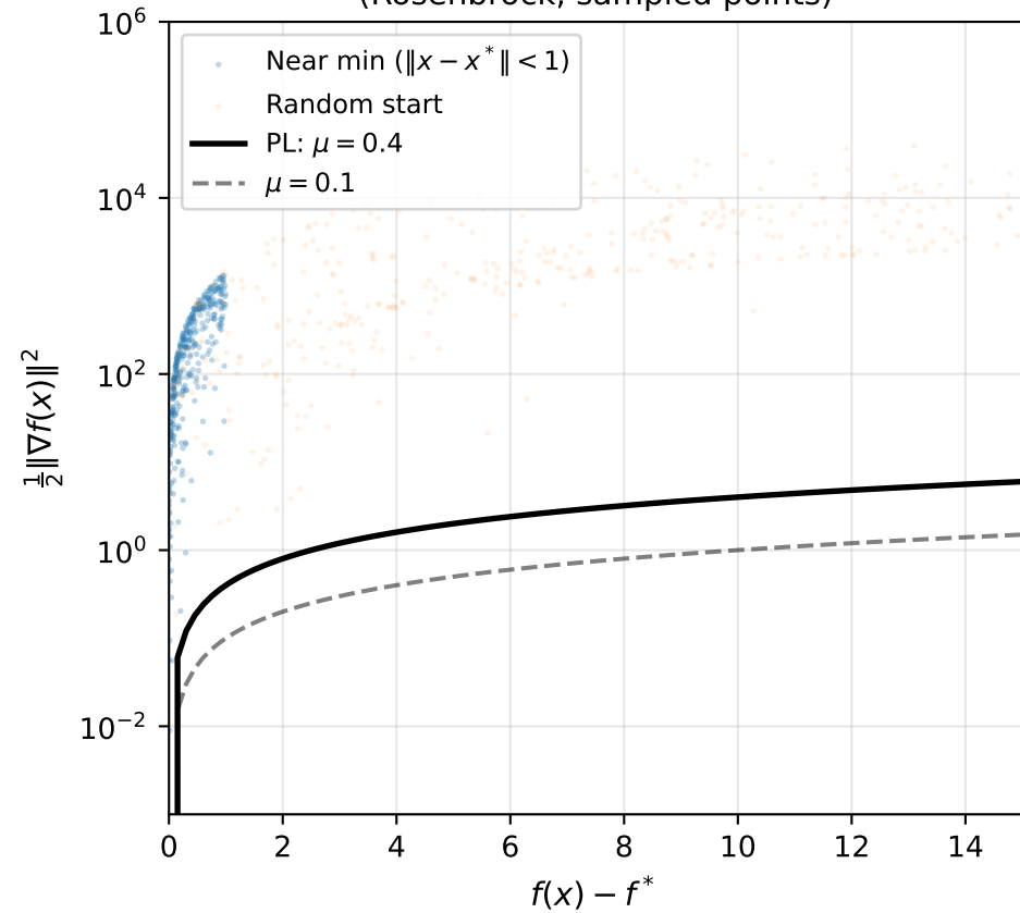
PL Condition Verification (Rosenbrock, sampled points)
