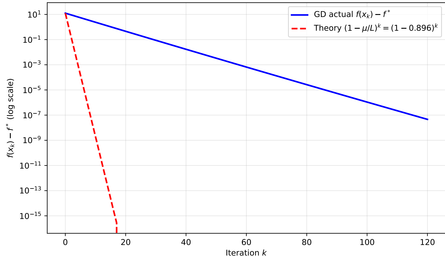
Q1: GD Convergence vs Theory on Benchmark A ( \kappa = 1.12 )
