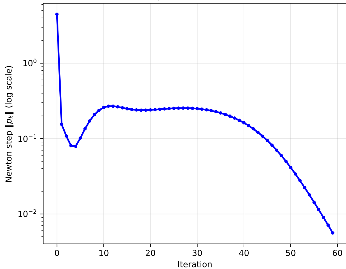
Q3: Newton Step Size (decrement) vs Iteration
