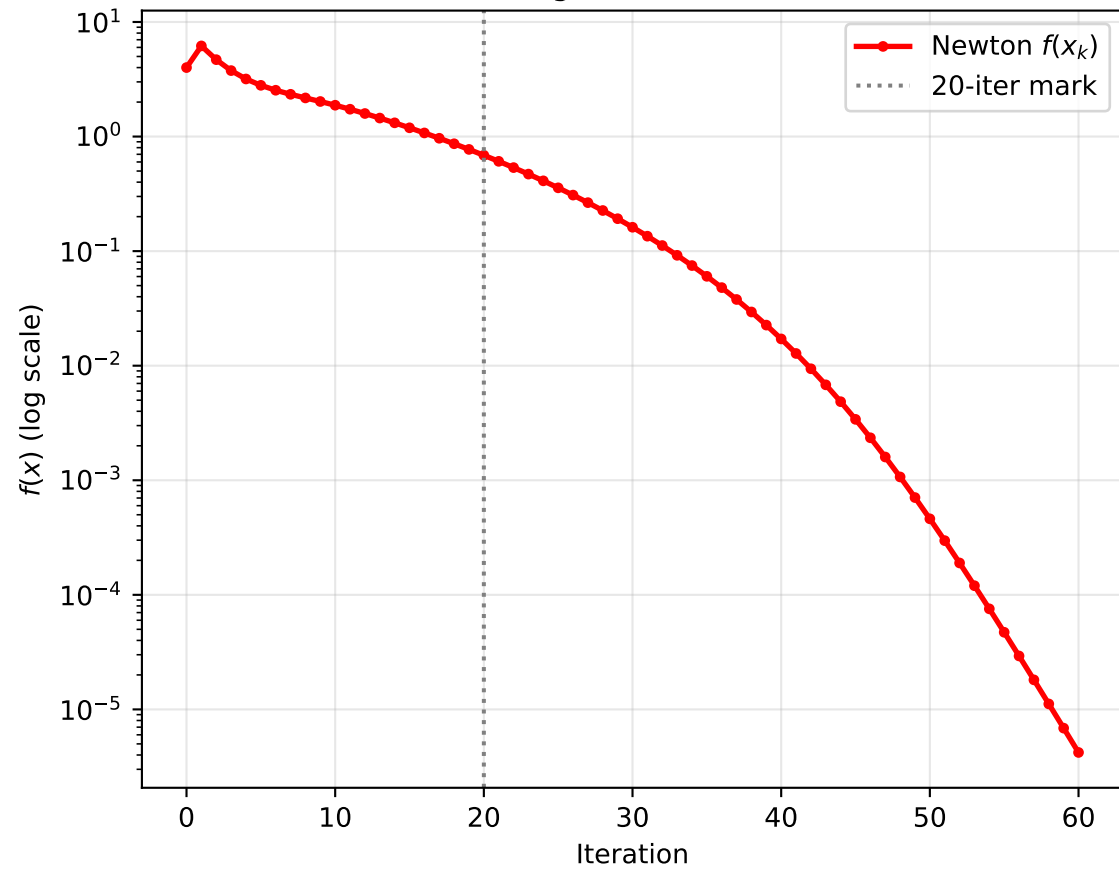
Q3: Newton's Convergence on Rosenbrock (60 iters)
