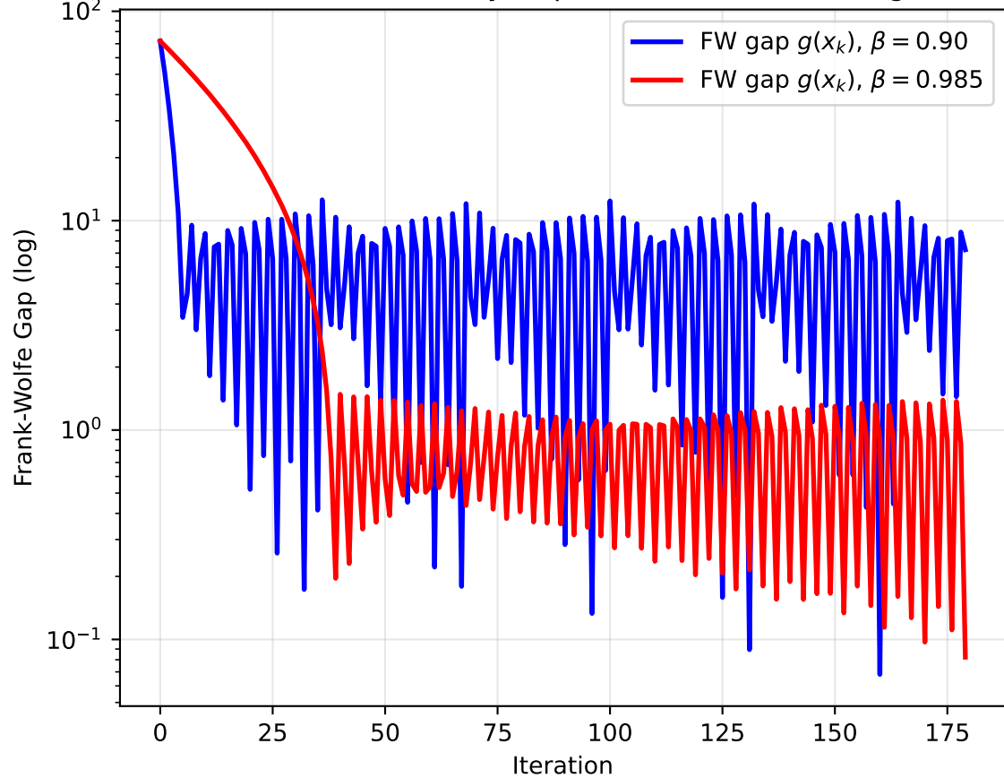
Q6-II: Frank-Wolfe Duality Gap (Certificate of Convergence)
