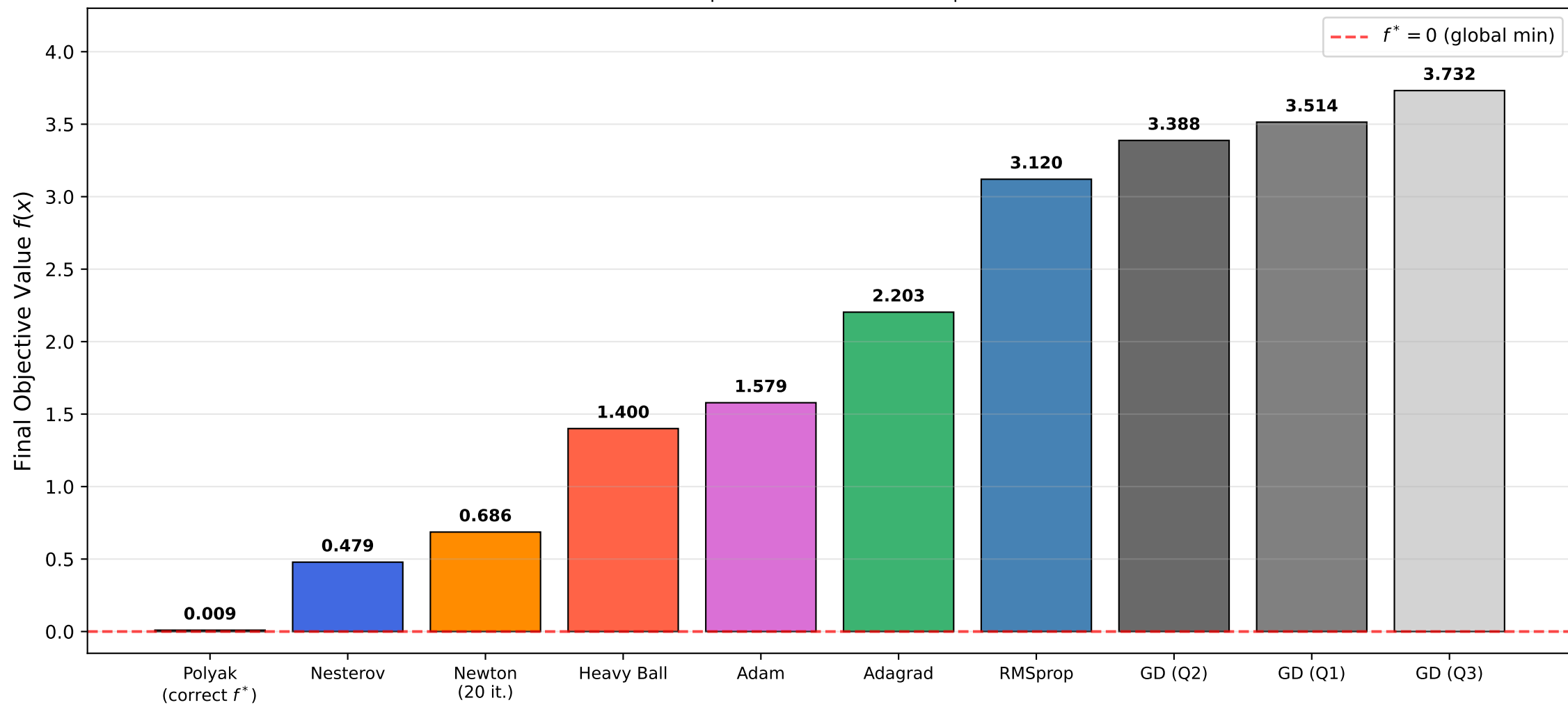
Benchmark C (Rosenbrock, f^* = 0 ): Final Objective Across All Methods
