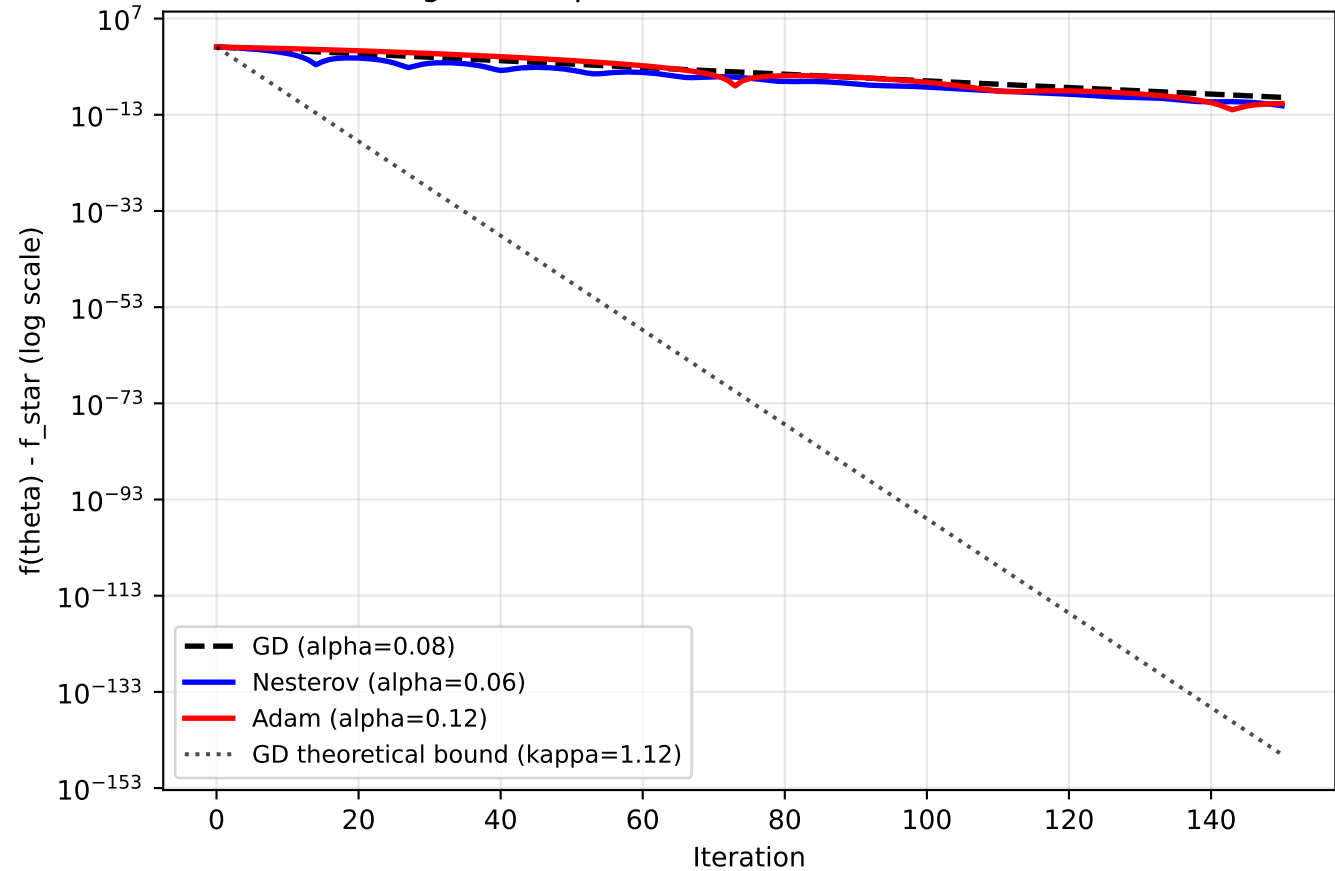
Convergence Gap vs Theoretical Bound (Benchmark A)
