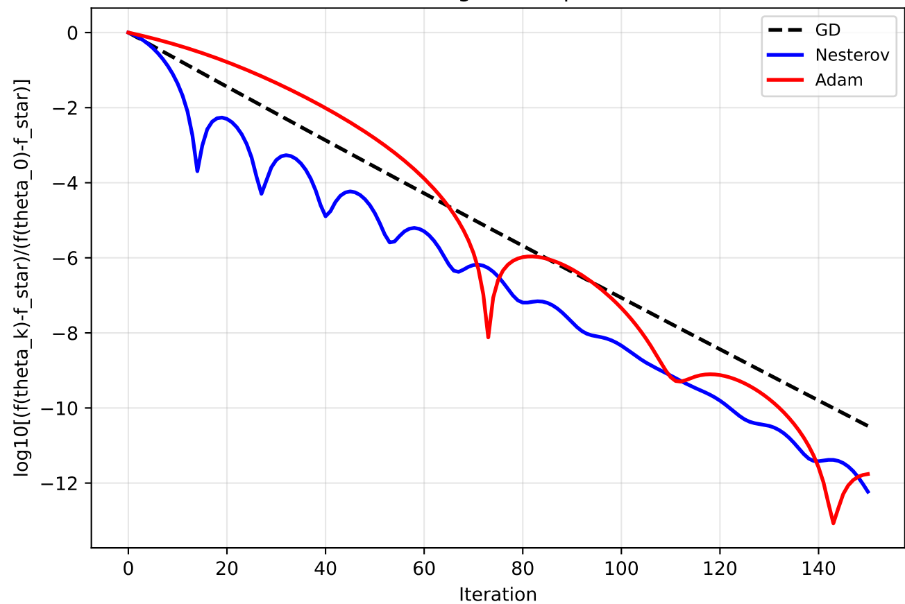
Normalised Convergence Gap (Benchmark A)
