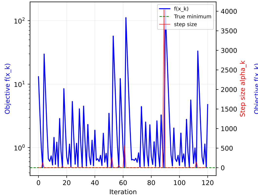
Benchmark A (Linear Reg.) ( f^*=0 wrong)
