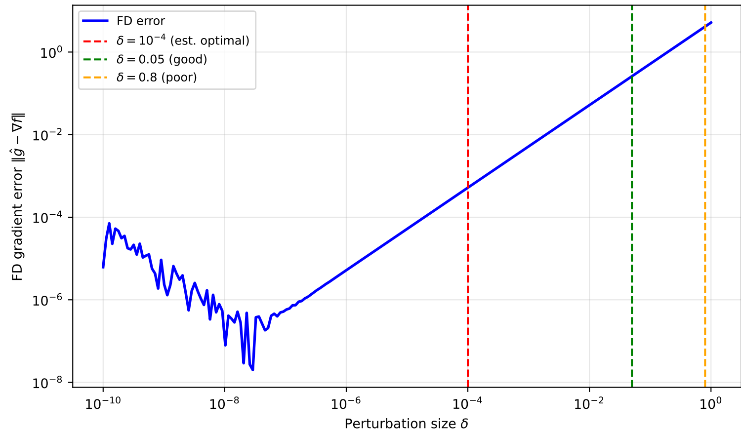
Q4: Finite Difference Error vs Perturbation Size (Benchmark B at $)
