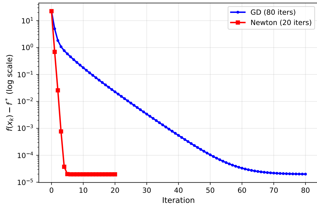
Excess Objective: Newton vs GD (Benchmark B)
