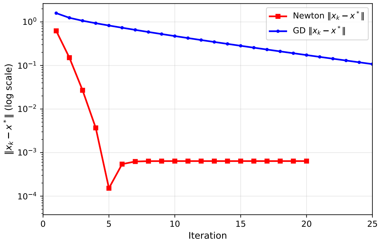
Distance to Optimum: Newton vs GD (Benchmark B)
