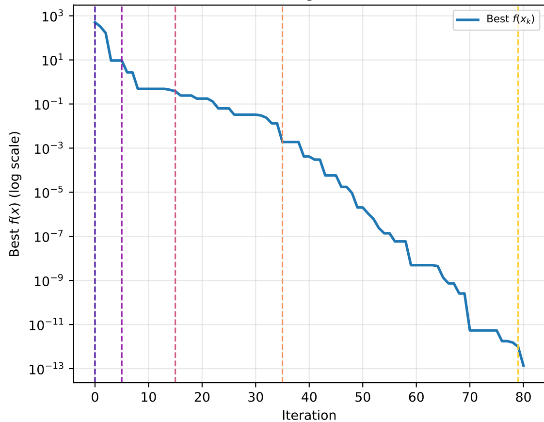
Nelder-Mead Convergence on Rosenbrock
