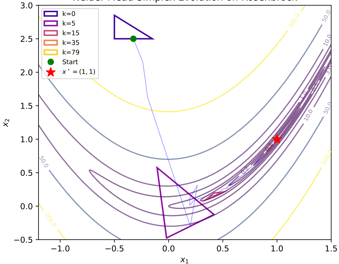
Nelder-Mead Simplex Evolution on Rosenbrock
