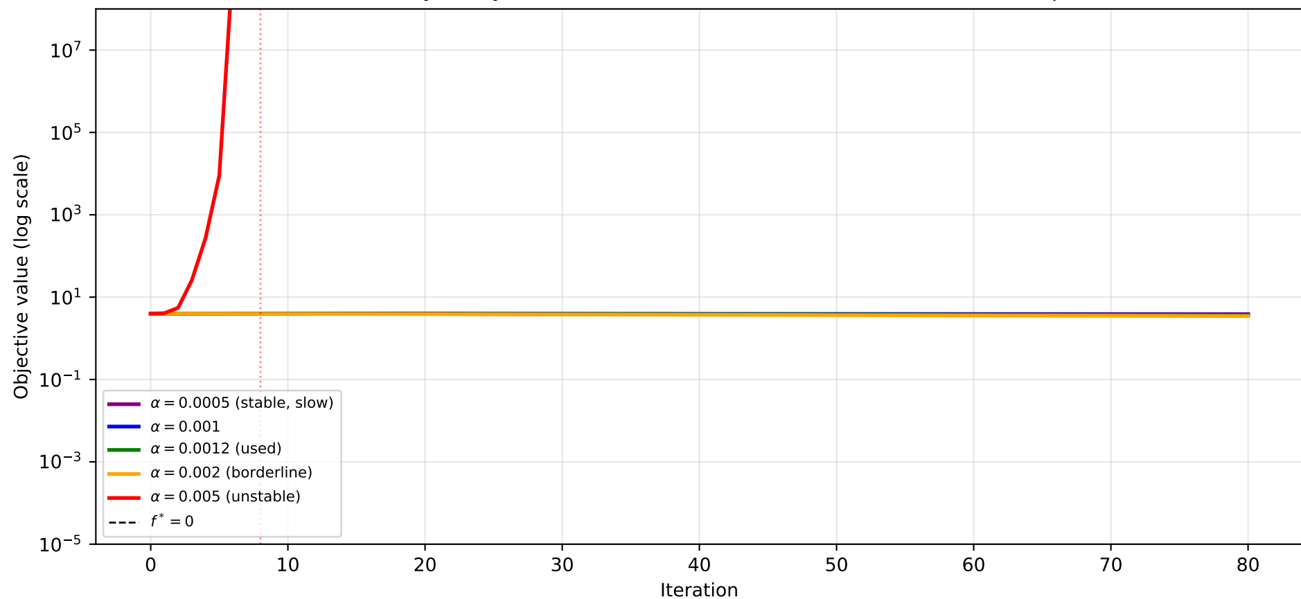
Q1: GD Stability Analysis on Benchmark C (Rosenbrock) — Effect of Step Size \alpha
