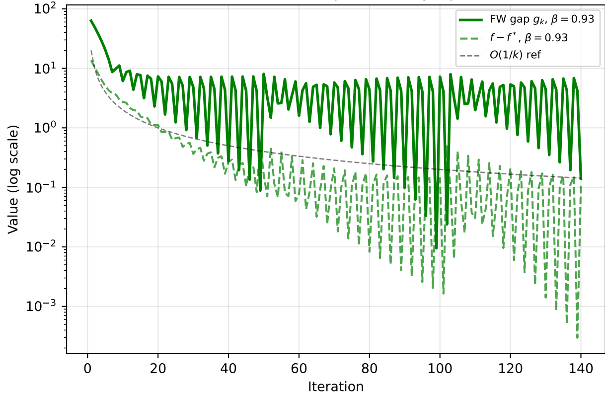
Q6-III: Frank--Wolfe Gap (Boundary Optimum)
