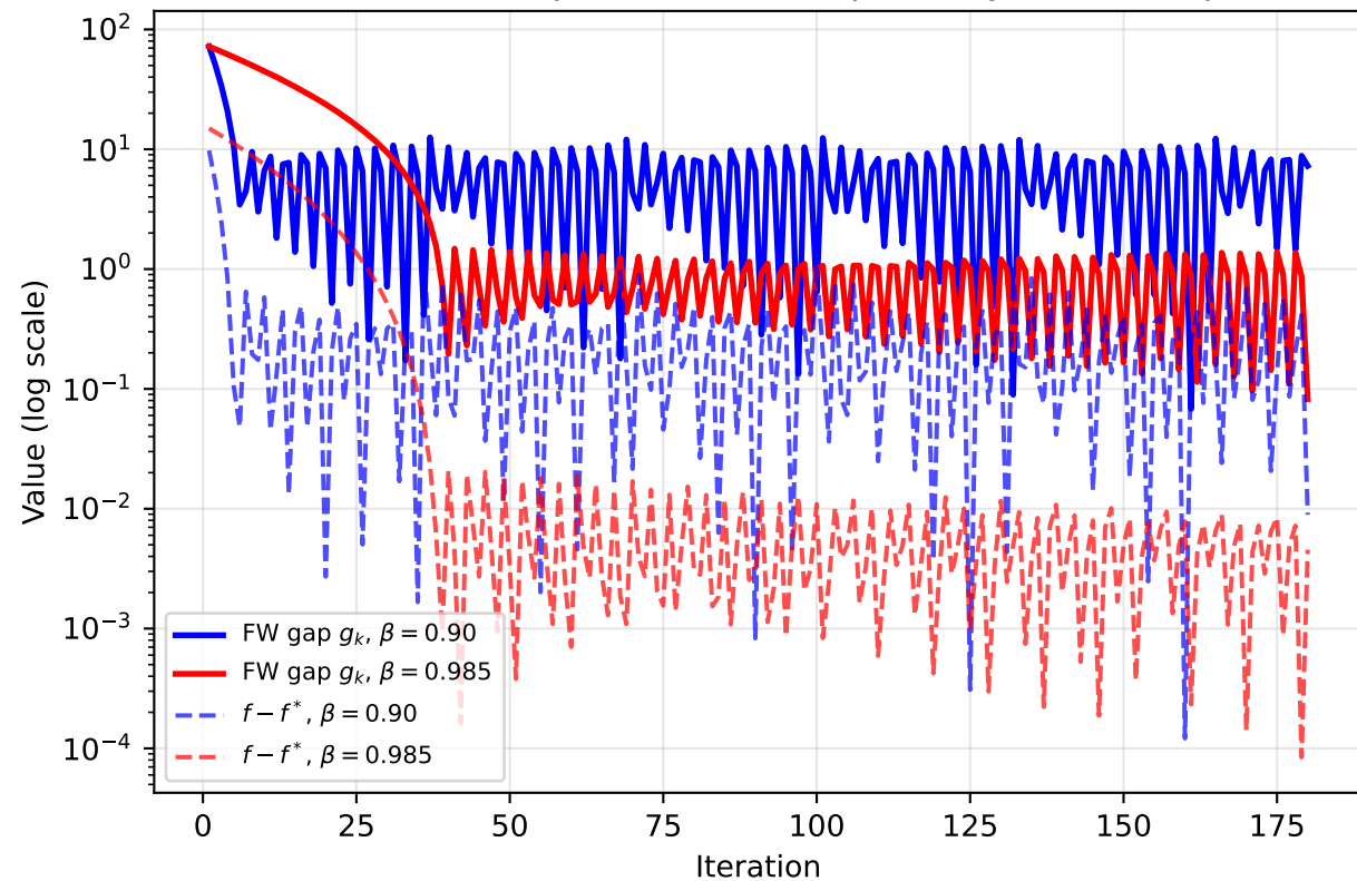
Q6-II: Frank--Wolfe Gap vs Primal Suboptimality (Interior Optimum)
