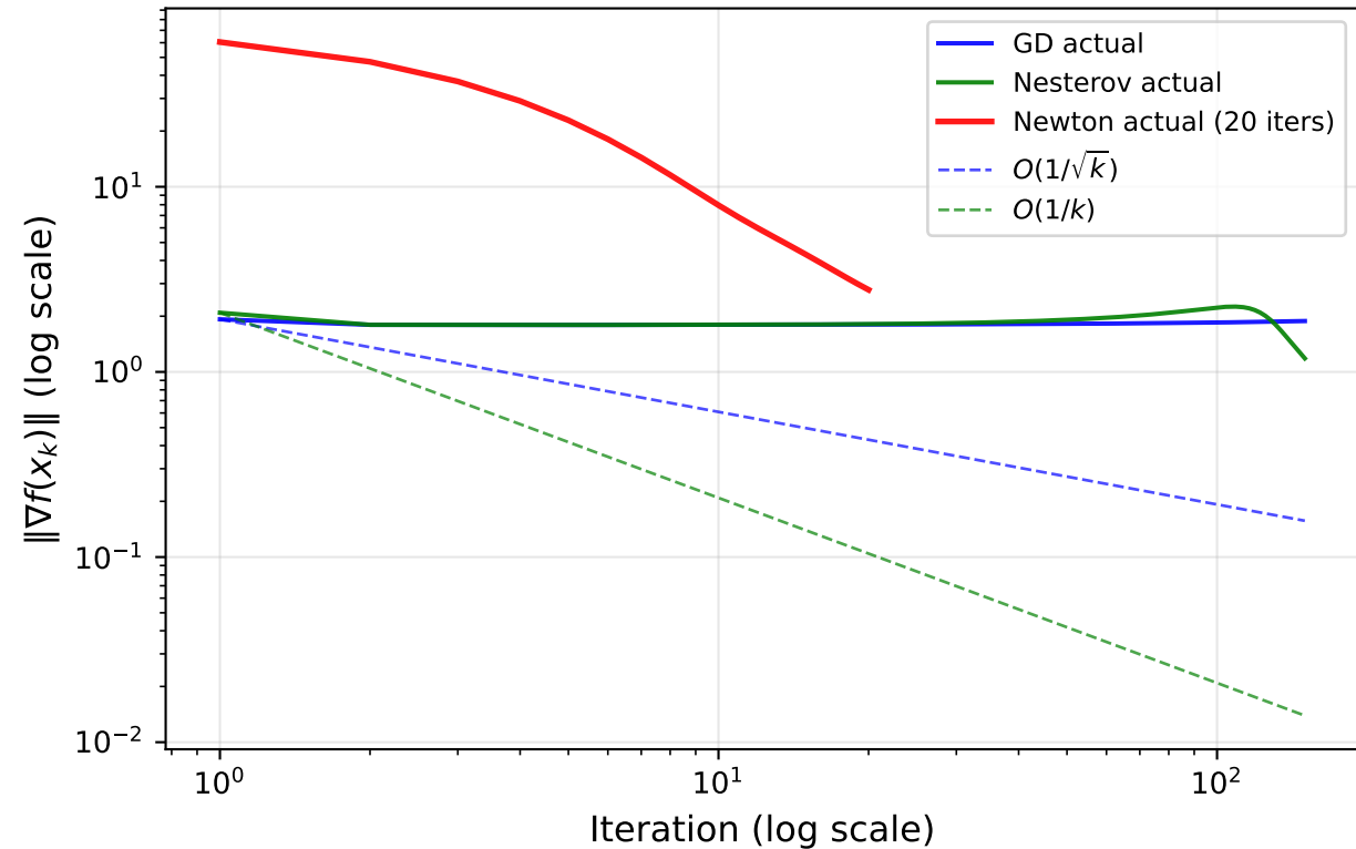
Log-Log: Gradient Norm Decay Rates
