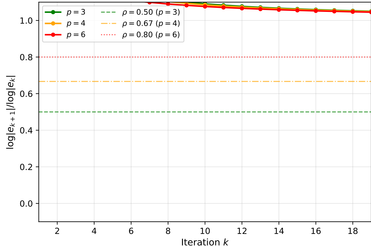
Linear Rate Constant \rho = (p - 2)/(p - 1)
