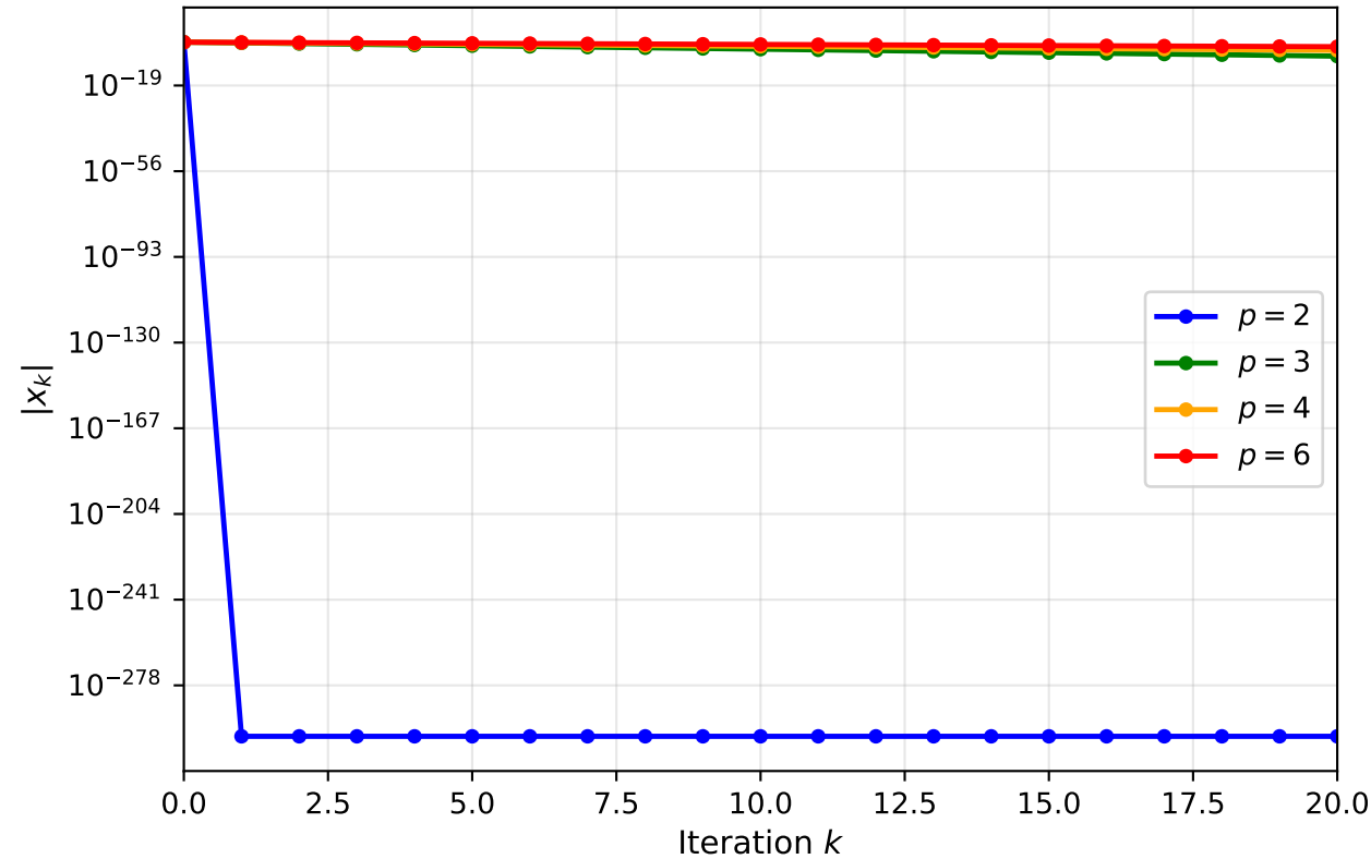
Newton's Method on g(x) = x^p : Iterates
