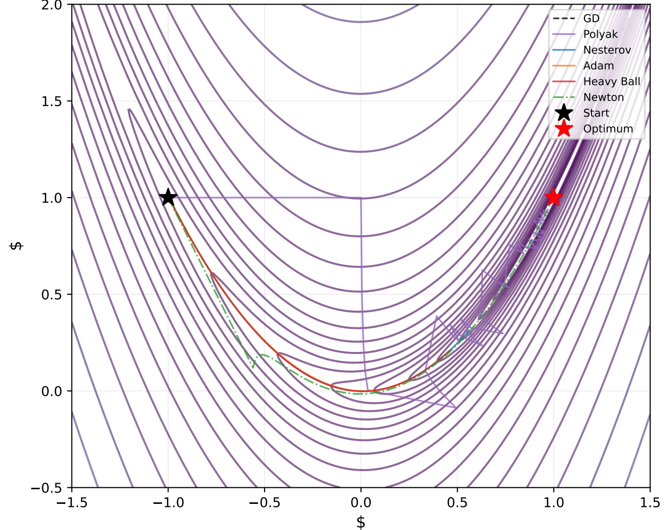
Rosenbrock: All Trajectories
