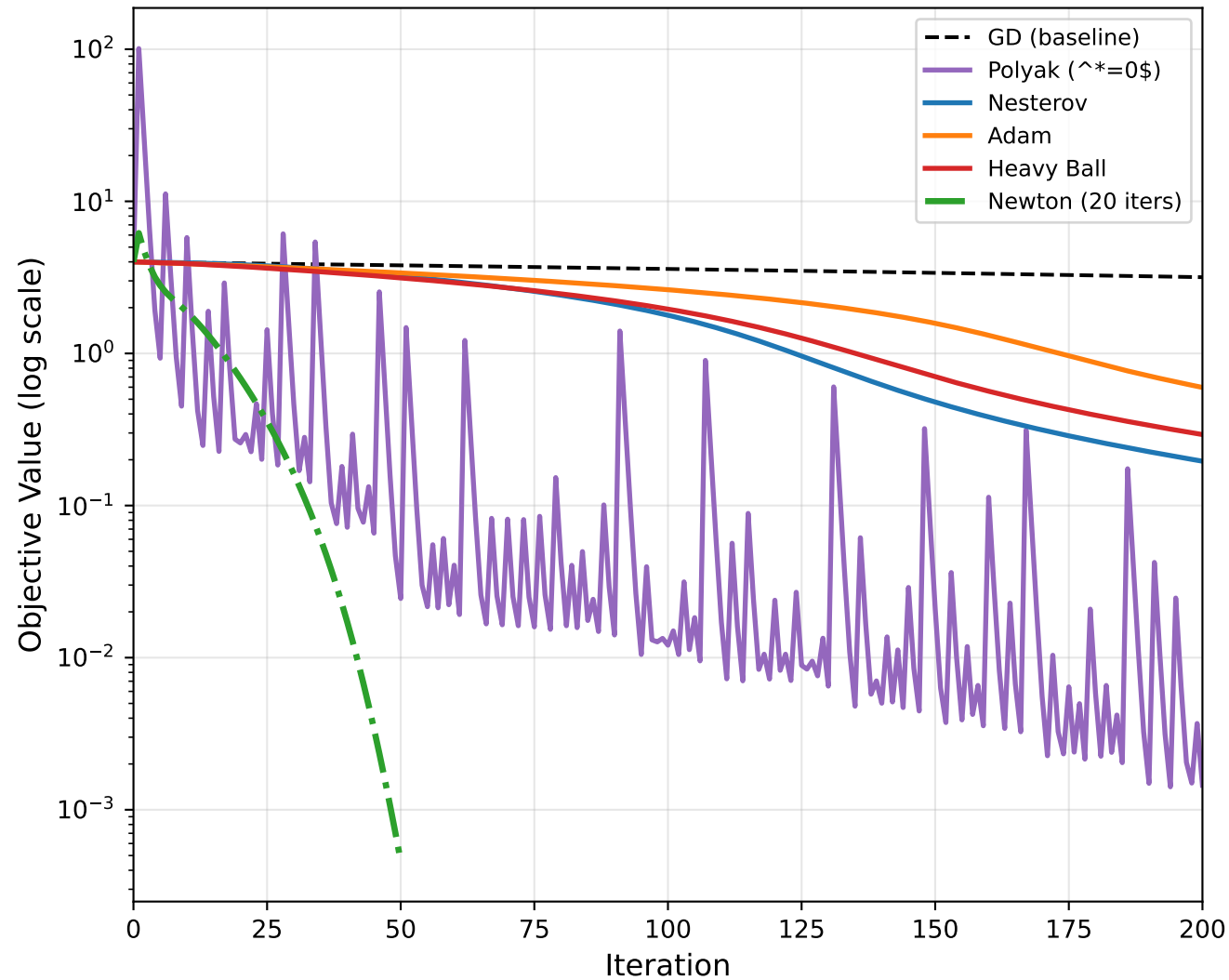
Rosenbrock: All Methods Compared
