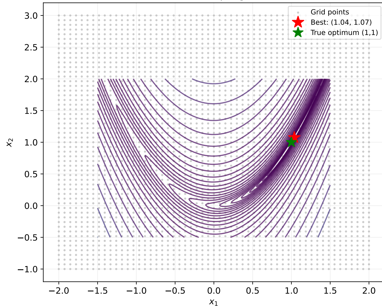
Q4B: Grid Search Sampling — Rosenbrock
