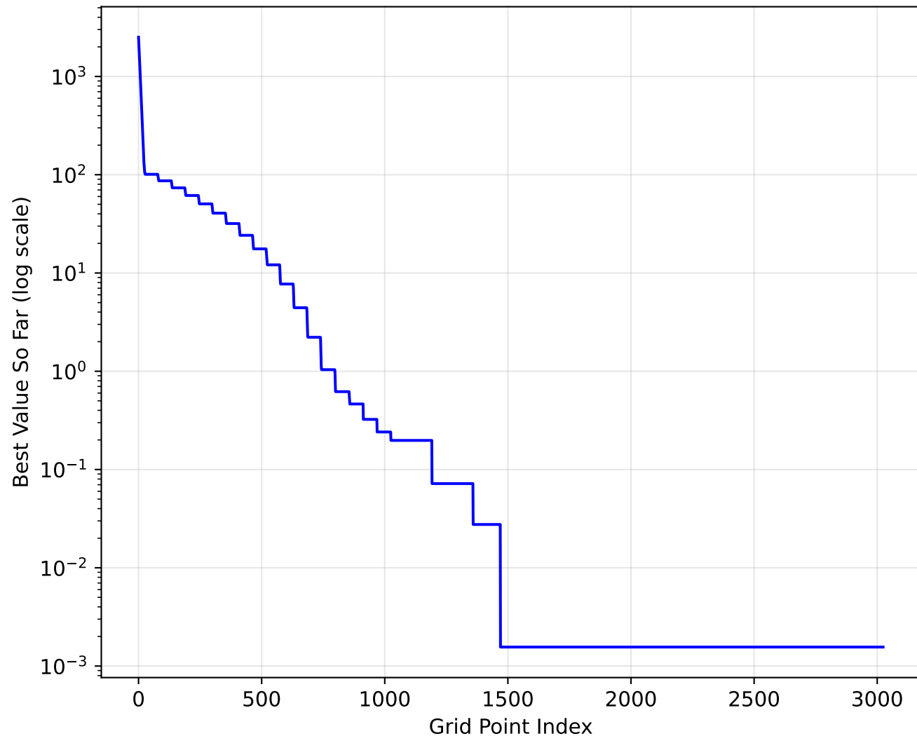
Q4B: Grid Search Best-So-Far (best f = 0.0016 )
