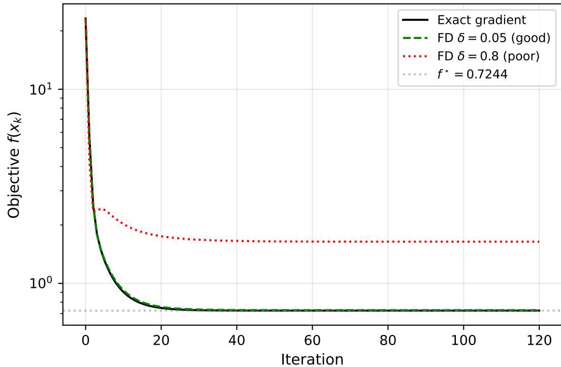
GD Convergence: Exact vs FD Gradient (Benchmark B)
