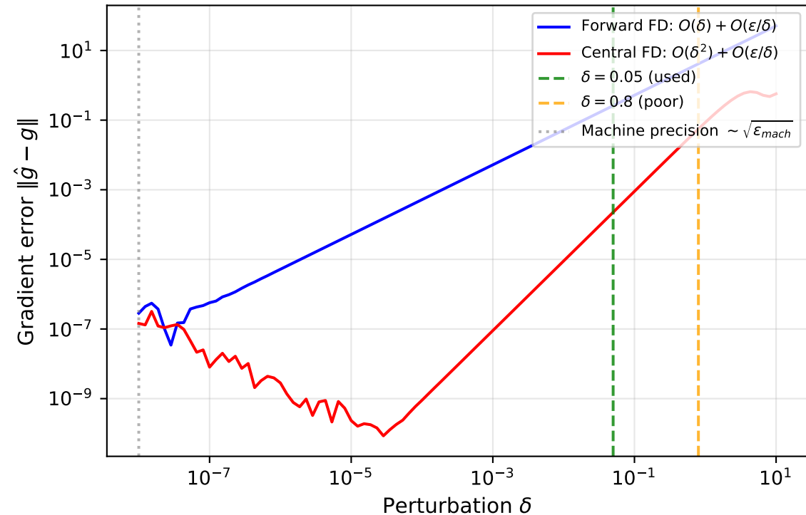
FD Gradient Error vs Perturbation \delta (Benchmark B, x_0 = (-1, 4) )
