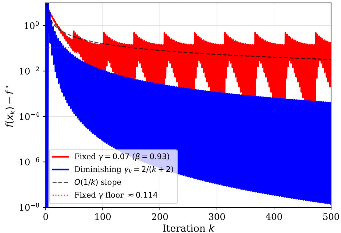
Fixed vs. Diminishing Schedule (500 iterations)
