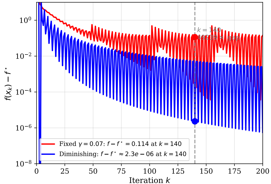
First 200 Iterations: Schedule Impact
