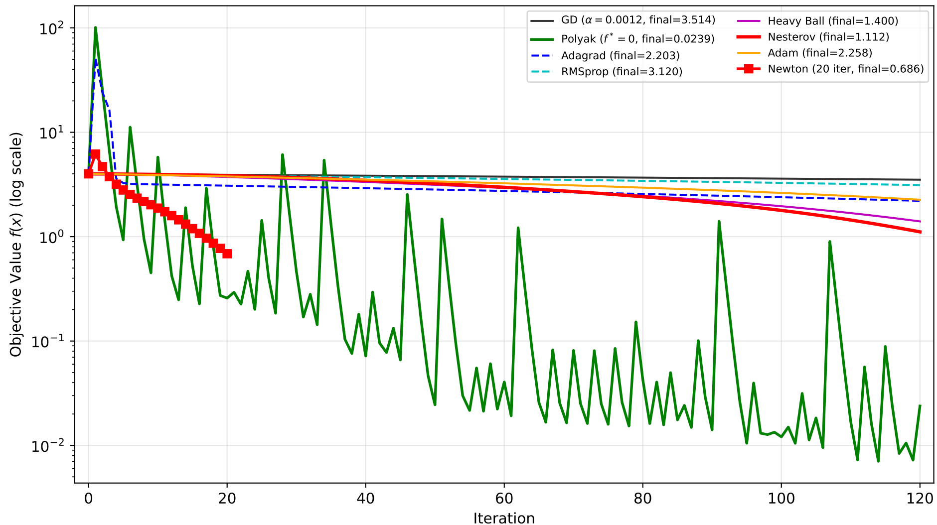
All Methods — Benchmark C (Rosenbrock, \kappa \approx 2508 )
