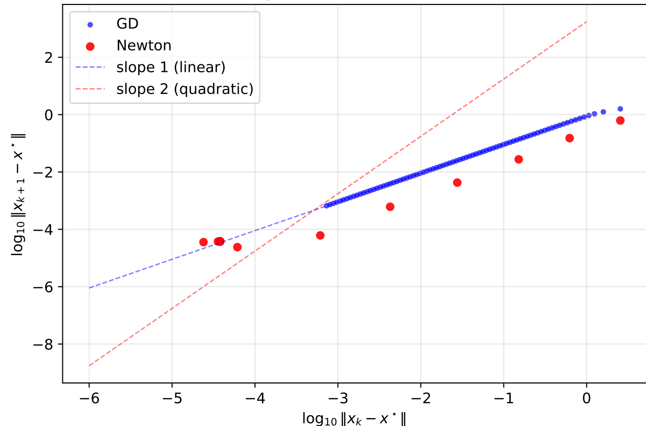
Q3: Convergence Order Plot (Benchmark B)
