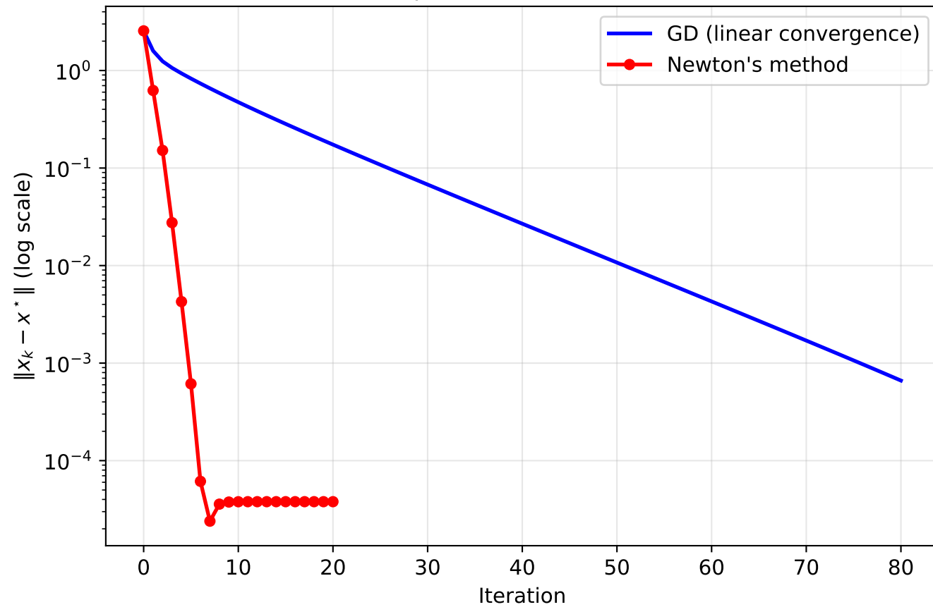
Q3: Distance to Optimum vs Iteration (Benchmark B)
