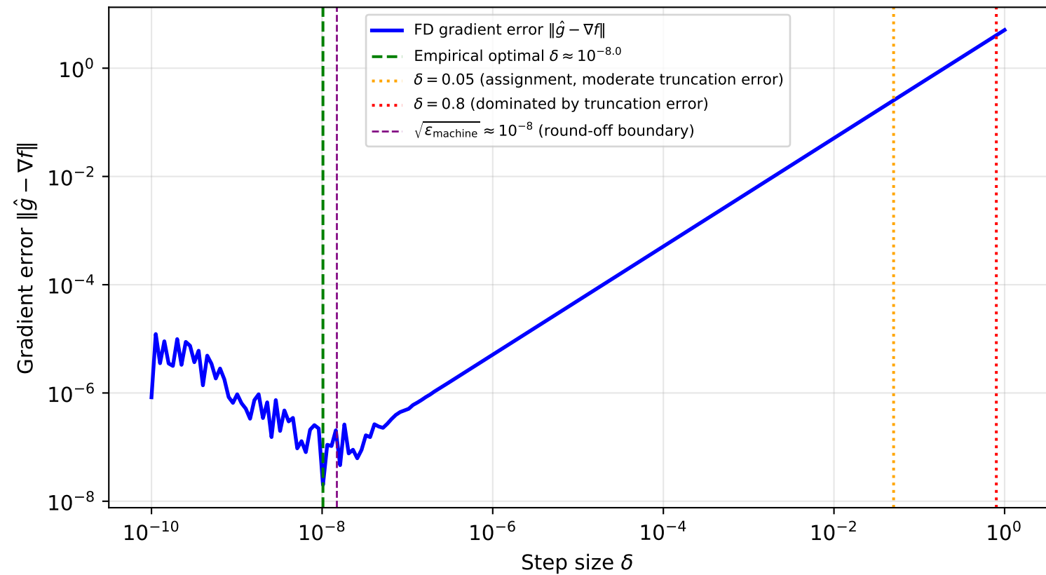
Q4A: FD Gradient Error vs Step Size at x = (0, 3) (Benchmark B, Forward Difference)
