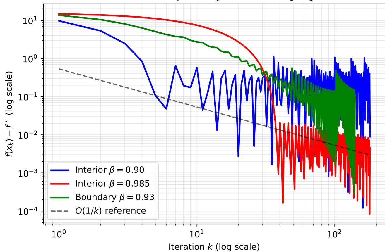
Q6: FW Suboptimality f(x_k) - f^* (log-log)
