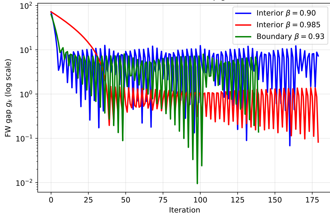
Q6: Frank--Wolfe Linearisation Gap g_k = \nabla f(x_k)^T(x_k - z_k)
