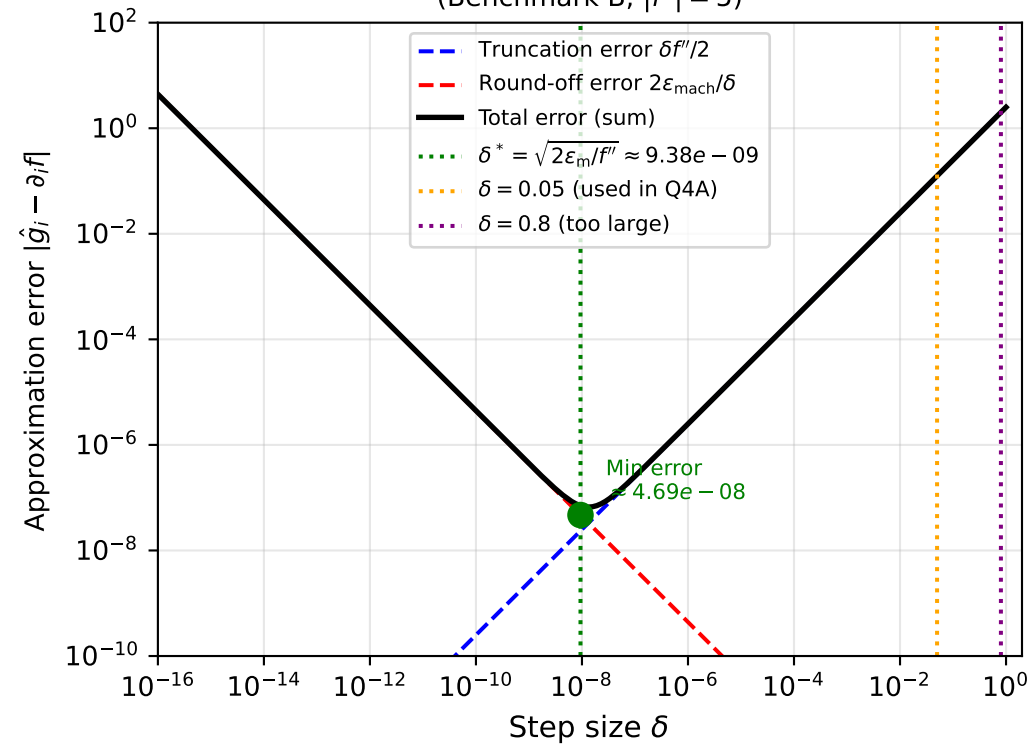
FD error decomposition (Benchmark B, |f''| = 5 )
