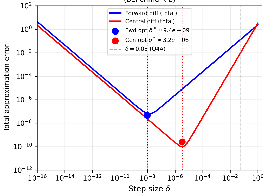
Forward vs. Central differences (Benchmark B)
