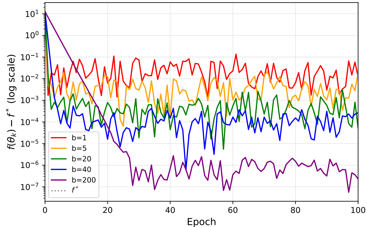
Mini-Batch SGD: Convergence vs Batch Size ( \alpha=0.06 )
