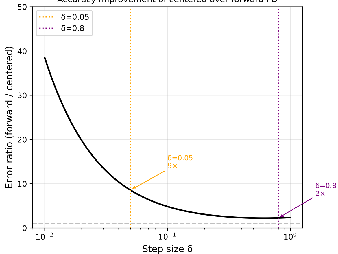
Accuracy improvement of centered over forward FD
