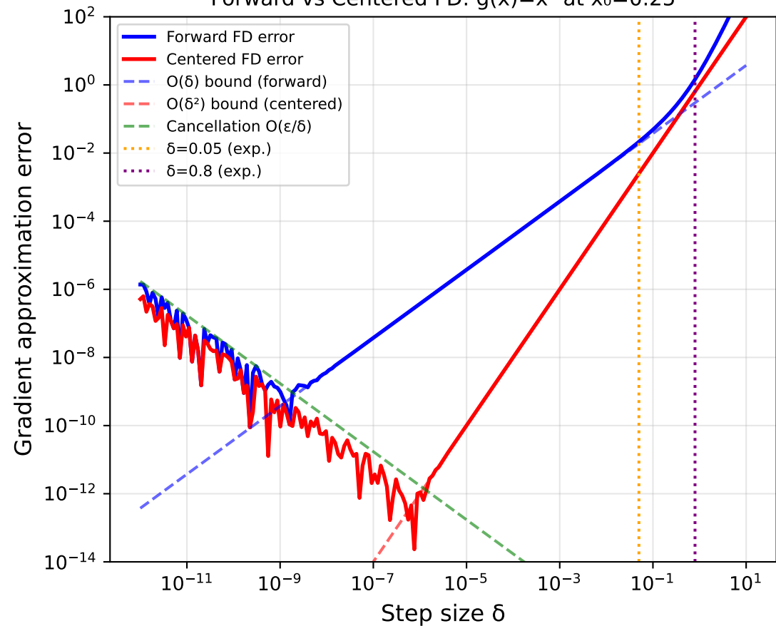
Forward vs Centered FD: g(x)=x^4 at x_0=0.25
