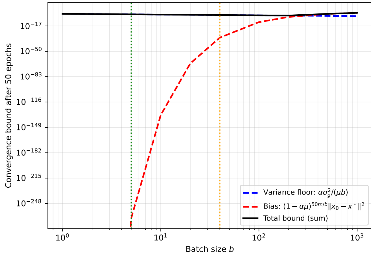
SGD: Bias--Variance Trade-off vs Batch Size
