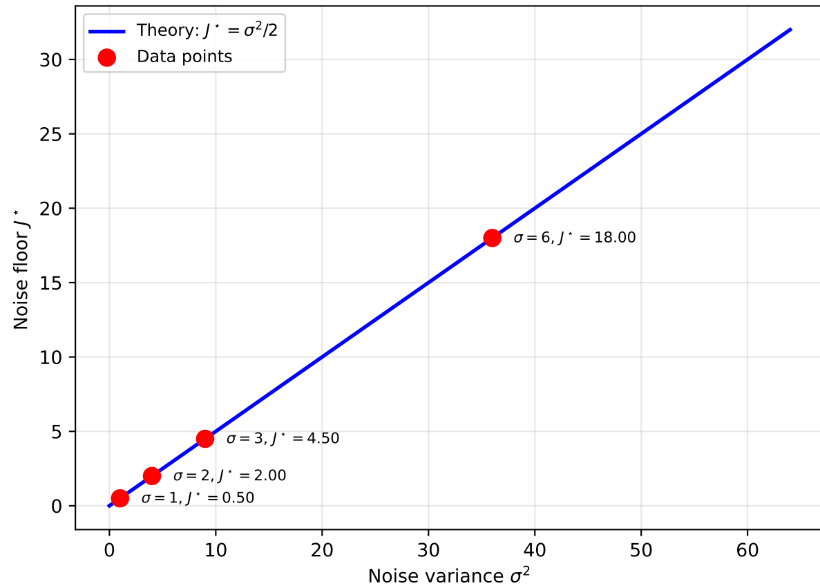
Noise Floor Scaling: J^* = \sigma^2/2
