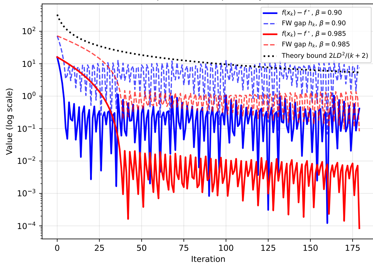
Q6: FW Gap h_k vs Sub-optimality f(x_k) - f^*
