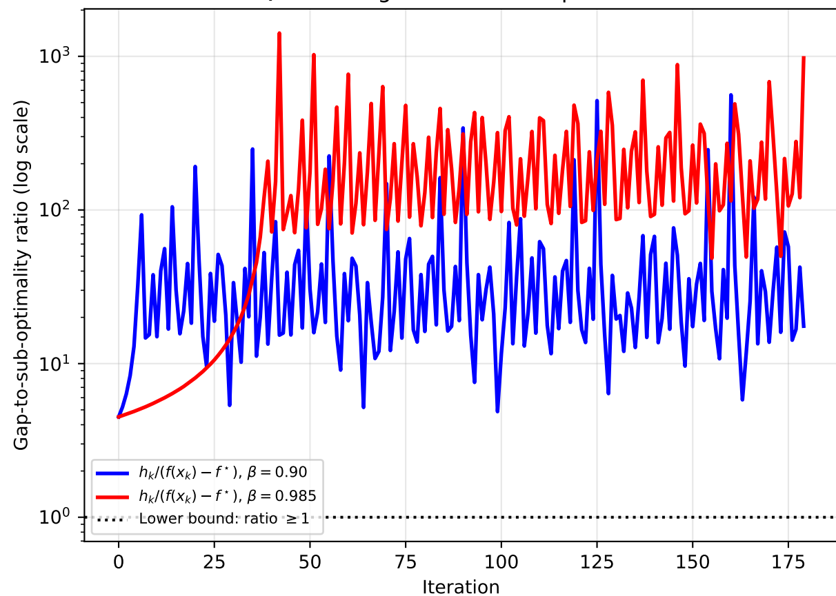
Q6: How Tight is the FW Gap Bound?
